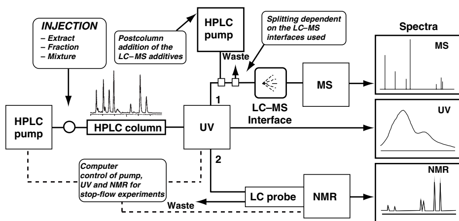
FIGURE 1.13 Schematic representation of the instrumentation used for LC-UV-MS (1) and LC-UV-NMR (2) analyses.
