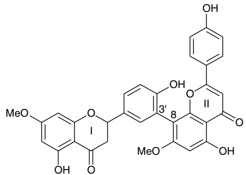
(15) Amentotaxus yunnanensis , rel. config., Ref. 44
