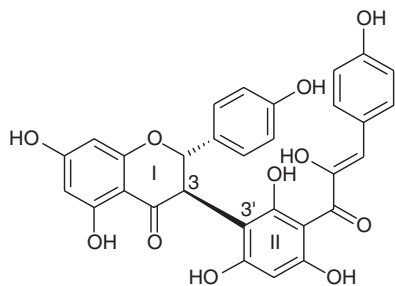
(85) Flavanone- \alpha -hydroxychalcone — Berchemia zeyheri , abs. config., Ref. 37
