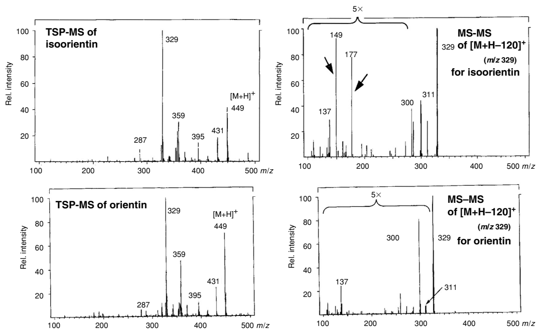
FIGURE 1.11 Online mass spectra of isoorientin ( 1 ) and orientin ( 2 ) in the TSP mode. The respective TSP MS–MS (CID) analyses of the parent [M + H - 120]^+ ( m/z 329) ions are also shown.
