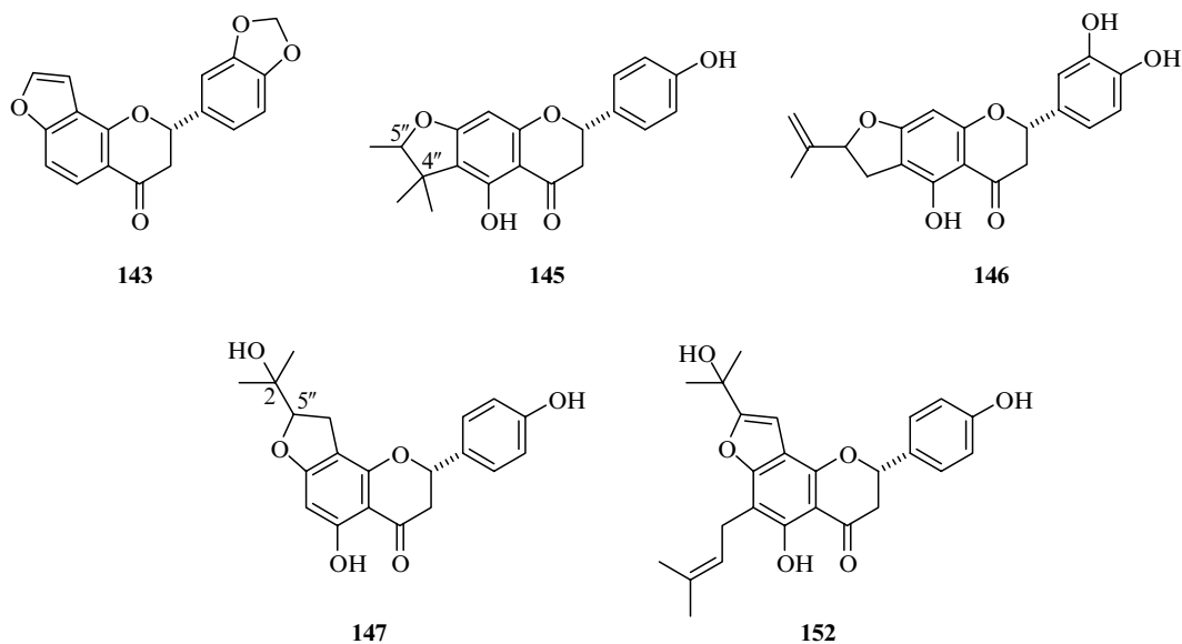
FIGURE 15.4 Examples of furanoflavanones.
