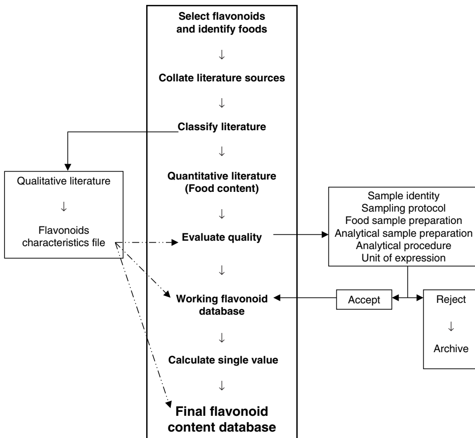
FIGURE 4.1 Schematic of selection and evaluation processes used to compile the flavonoid database.
