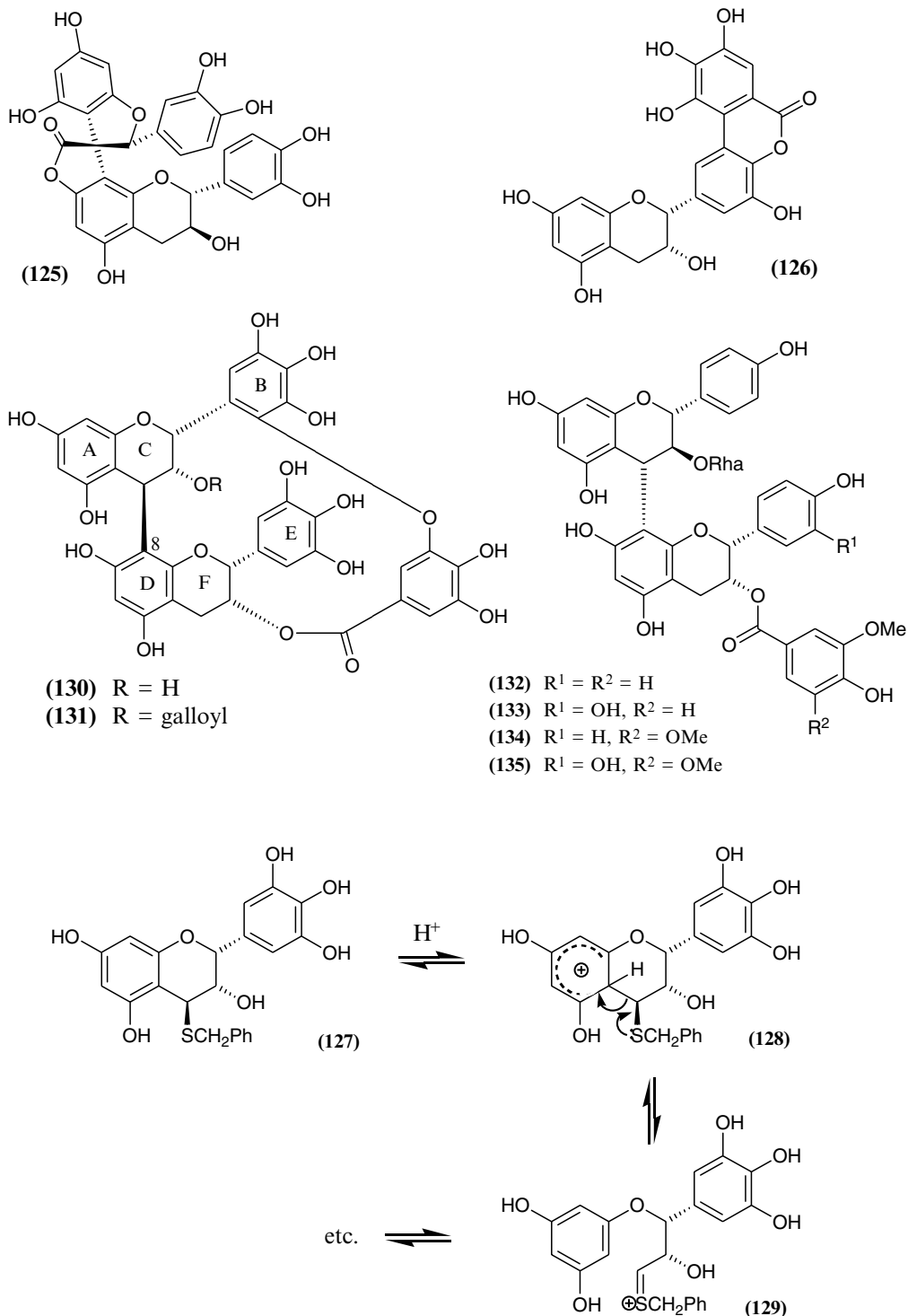
FIGURE 11.11 Structures of compounds 125–135 including Scheme 11.4: Proposed route to the acid-catalyzed cleavage of the C 4 –C 10 bond in C-4 thiobenzylflavan-3-ols.
