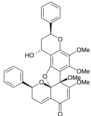
(134) 6''-Demethoxynecalycopteronone Calycopterus floribunda , abs. config., Ref. 104
