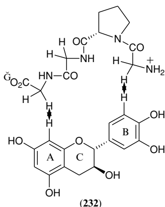
(232)
