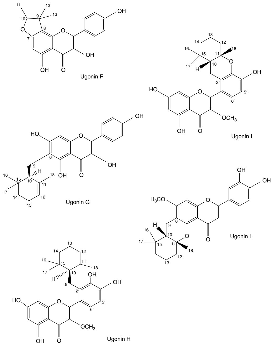
FIGURE 12.11 Flavonoids from Helminthostachys .
