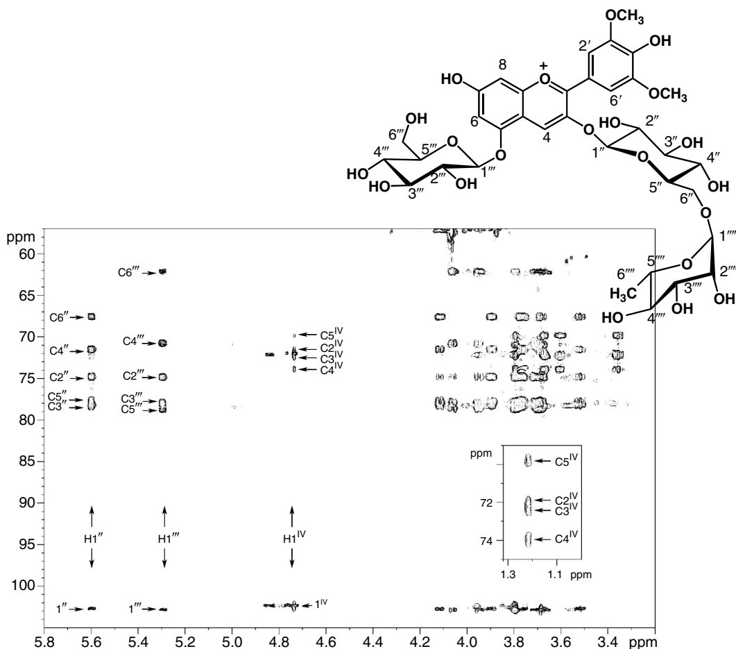
FIGURE 2.5 Region of the 2D ^1\text{H} - ^{13}\text{C} gs-HSQC-TOCSY spectrum of malvidin 3- O -(6''- O - \alpha -rhamnopyranosyl)- \beta -glucopyranoside)-5- O - \beta -glucopyranoside showing crosspeaks of most of the sugar signals. In this spectrum, each proton/carbon correlation shows crosspeaks to all ^1\text{H} and ^{13}\text{C} resonances belonging to the same spin system. The expanded region (boxed) reveals the correlation between H-6 IV and the carbons of the terminal rhamnose unit. 176
