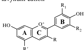
Flavylium cation
