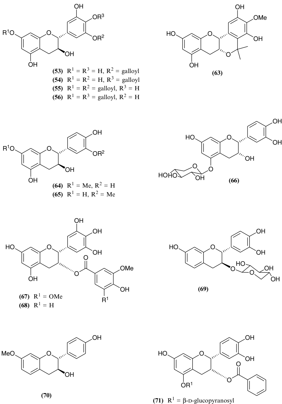
FIGURE 11.5 Structures of compounds 53–56 and 63–71.
