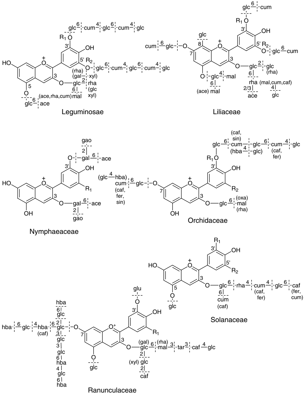
FIGURE 10.15 The structures represent a general presentation of all the anthocyanins identified in each of the families Leguminosae, Liliaceae, Nymphaeaceae, Orchidaceae, Ranunculaceae, and Solanaceae. See Table 10.2 for abbreviations.
