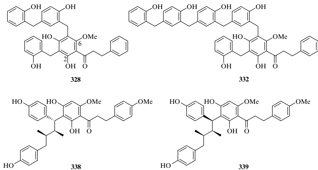
FIGURE 16.18 C-Benzylated dihydrochalcones and dihydrochalcone-lignan conjugates (see Table 16.12).
