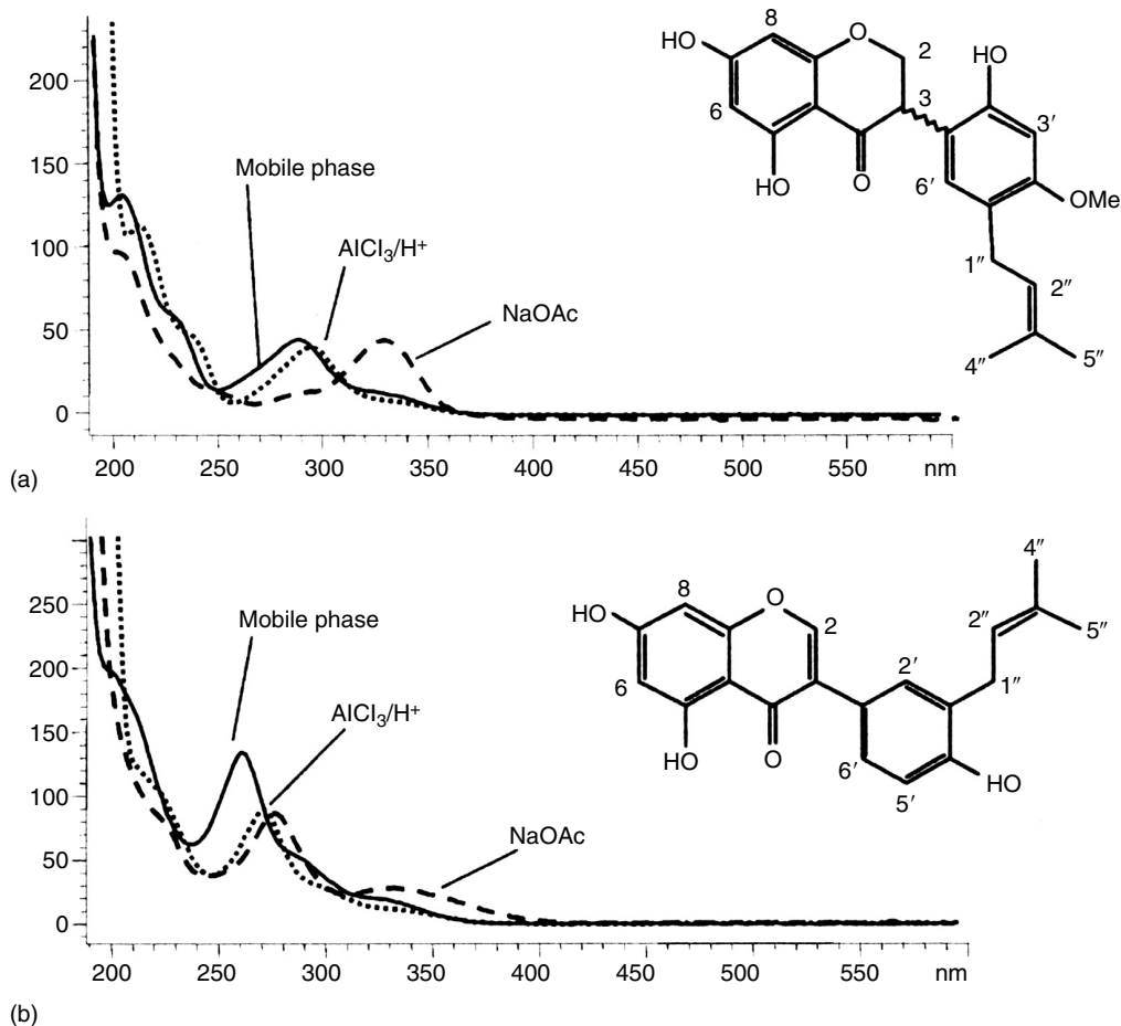
FIGURE 2.20 Complementary UV-DAD and shifted UV-DAD spectra with postcolumn addition of shift reagents of an isoflavanone (a) and an isoflavone (b) recorded online. The weak base NaOAc and acidic AlCl 3 , respectively, were used as shift reagents. The shifted UV spectra are superimposed on the original spectra for each compound. The observed shifts provide information about the flavonoid substitution in accordance to the rules established for pure compounds. (Modified from Wolfender, J.-L., Ndjoko, K., and Hostettmann, K., J. Chromatogr. A , 1000, 437, 2003. Copyright 2003 Elsevier Science B.V. With permission.)
