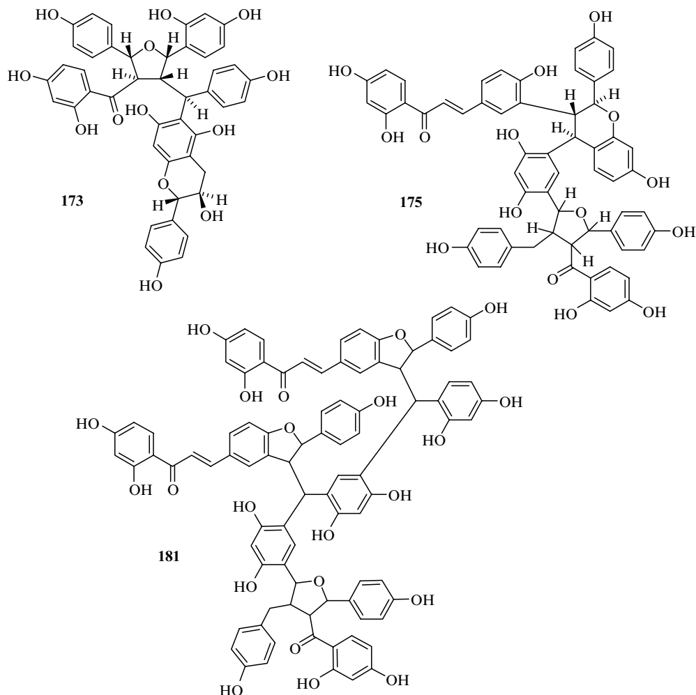
FIGURE 16.9 Chalcone dimers, heterodimers, and oligomers (see Table 16.4).
