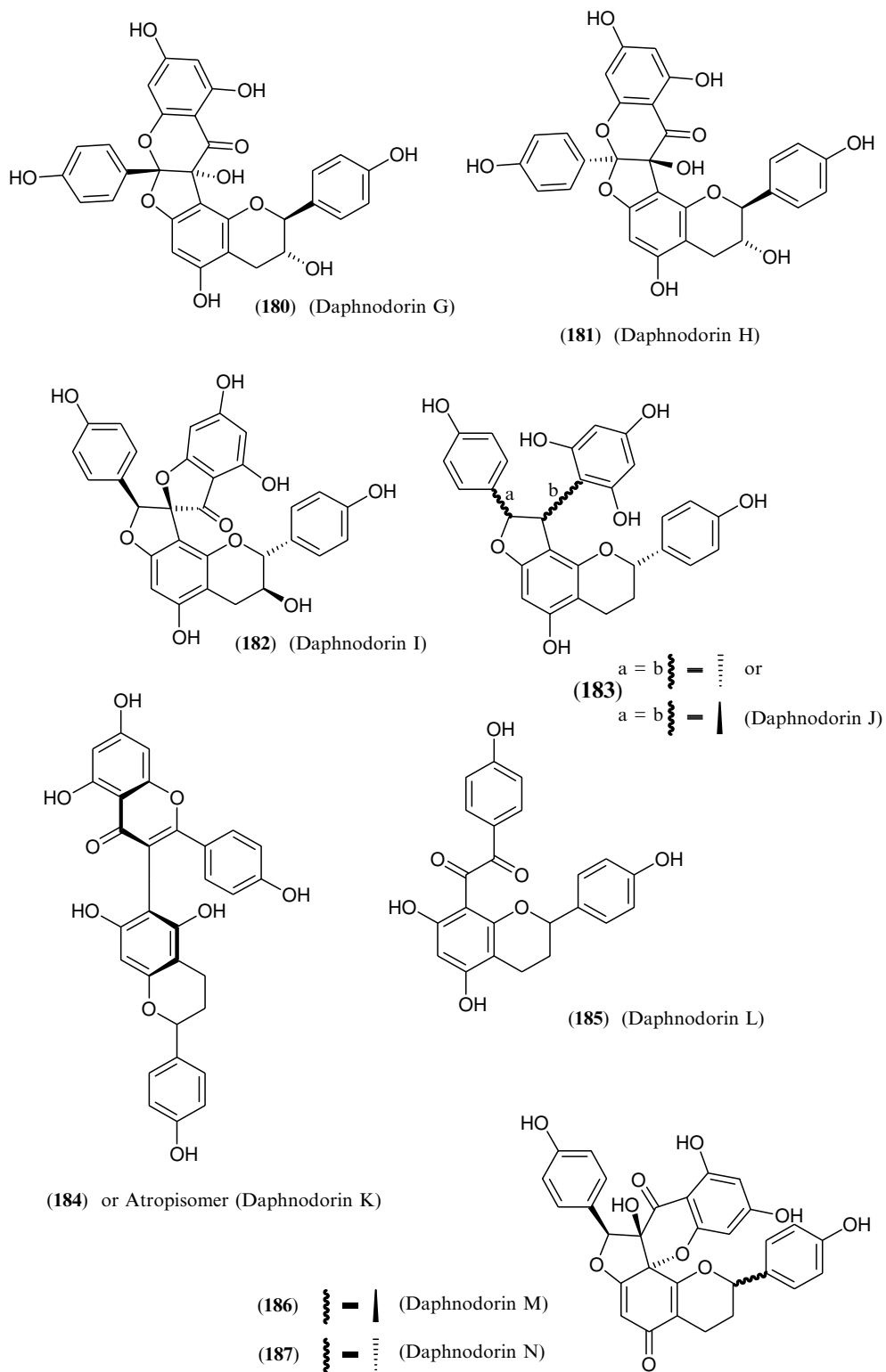
FIGURE 11.18 Structures of compounds 180–187.
