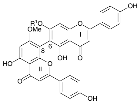
(2) R 1 = Me — Ouratea spectabilis , Ref. 28 (3) R 1 = H — Ouratea hexasperma , Ref. 33
