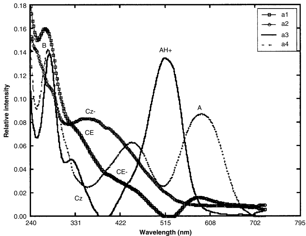
FIGURE 2.21 Spectral profiles recovered by the PARAFAC model at different pH values based on the deconvolution of UV–Vis absorption spectra, featuring the various anthocyanin secondary monomeric forms. (Reprinted from Levi, M.A.B. et al., Talanta , 62, 299, 2004. Copyright 2004 Elsevier Science B.V. With permission.)
