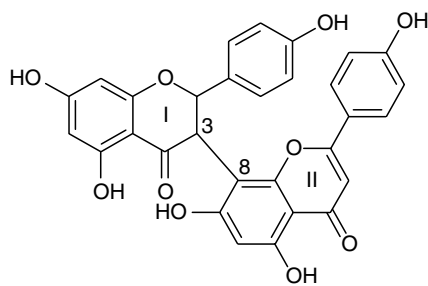
(95) Pancibiflavonol — Callophyllum paniciflorum , rel. config., Ref. 73
