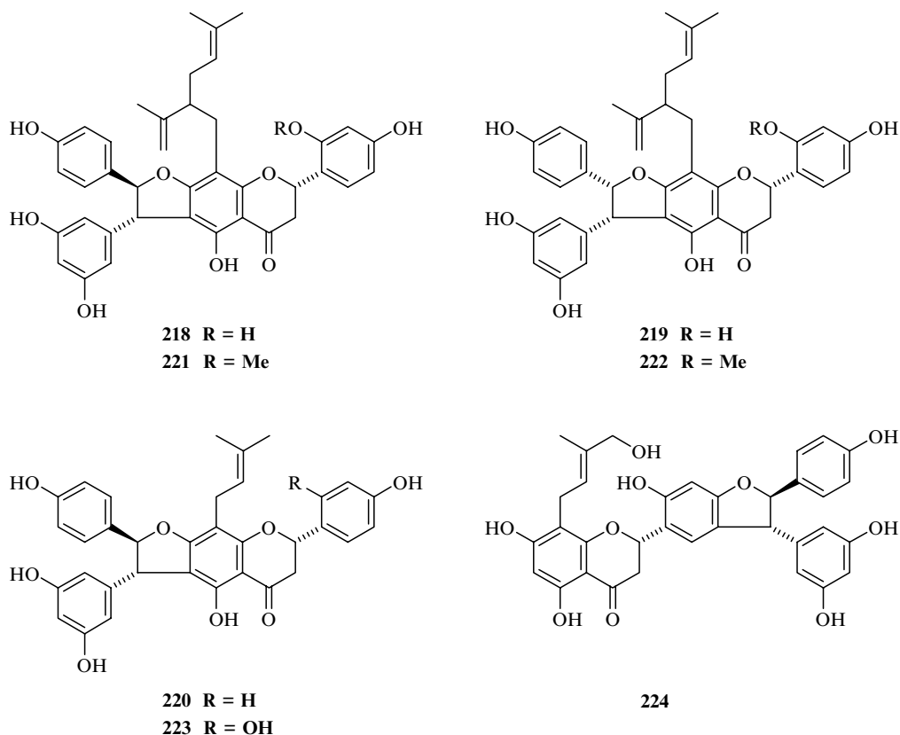
FIGURE 15.7 Flavanone-stilbenes.
