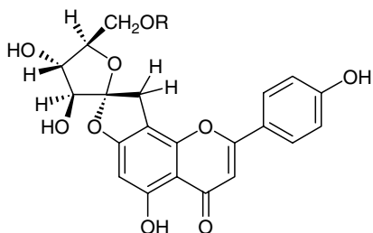
13.1 R = H
