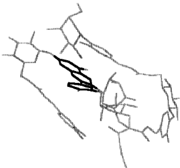
FIGURE 10.12 Structure of cyanidin 3-[6-(malonyl)glucoside]-7-[6-(caffeoyl)glucoside]-3'-[6-(4-(6-(4-(glucosyl)caffeoyl)glucosyl)caffeoyl)glucoside] ( 258 ) optimized by molecular calculations. The anthocyanidin is represented in black, while substituents are drawn in gray. The acylated side chains attached to the 3'- and 7-positions of the chromophore interact favorably with the \pi -system of the central chromophore. (From Figueiredo, P. et al., Phytochemistry , 51, 125, 1999. With permission.)
