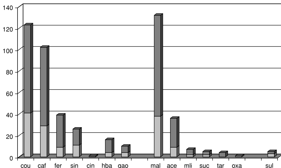
FIGURE 10.7 Numbers of anthocyanins containing the various acyl moieties identified in anthocyanins. The upper dark part of each bar represents the anthocyanins reported later than 1992. cou, p -coumaric acid; caf, caffeic acid; fer, ferulic acid; sin, sinapic acid; cin, 3,5-dihydroxycinnamic acid; hba, p -hydroxybenzoic acid; gao, gallic acid; mal, malonic acid; ace, acetic acid; mli, malic acid; suc, succinic acid; tar, tartaric acid; oxa, oxalic acid; sul, sulfate.
