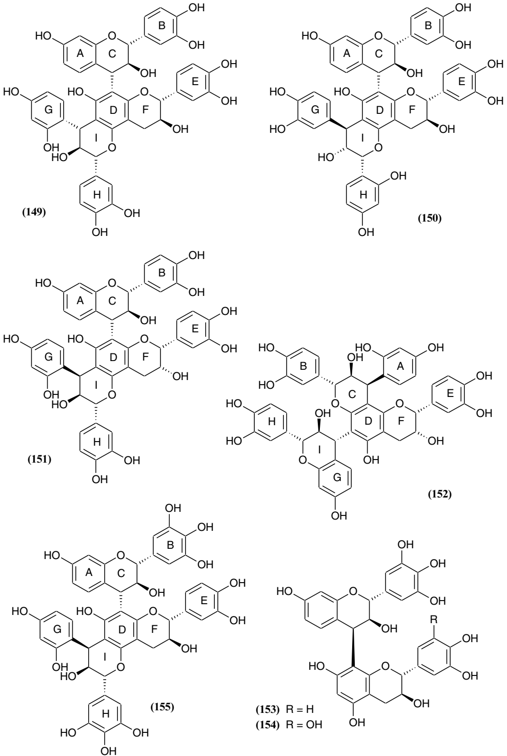
FIGURE 11.14 Structures of compounds 149–155.
