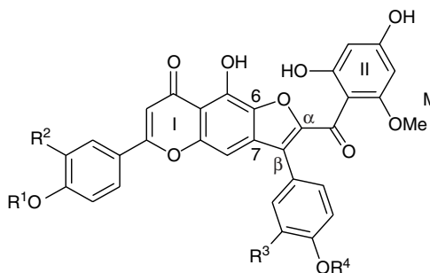
(87) R^1 = \text{Me} , R^2 = R^4 = \text{H} , R^3 = \text{OMe} } (88) R^1 = R^3 = \text{H} , R^2 = \text{OMe} , R^4 = \text{Me} } (89) R^1 = R^4 = \text{Me} , R^2 = \text{H} , R^3 = \text{OH} } — Aristolochia ridicula , Ref. 45
