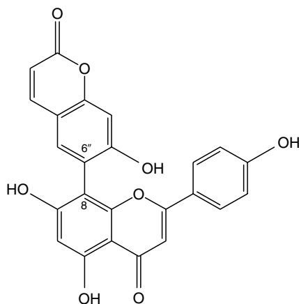
8-(6''-Umbelliferyl)-apigenin
