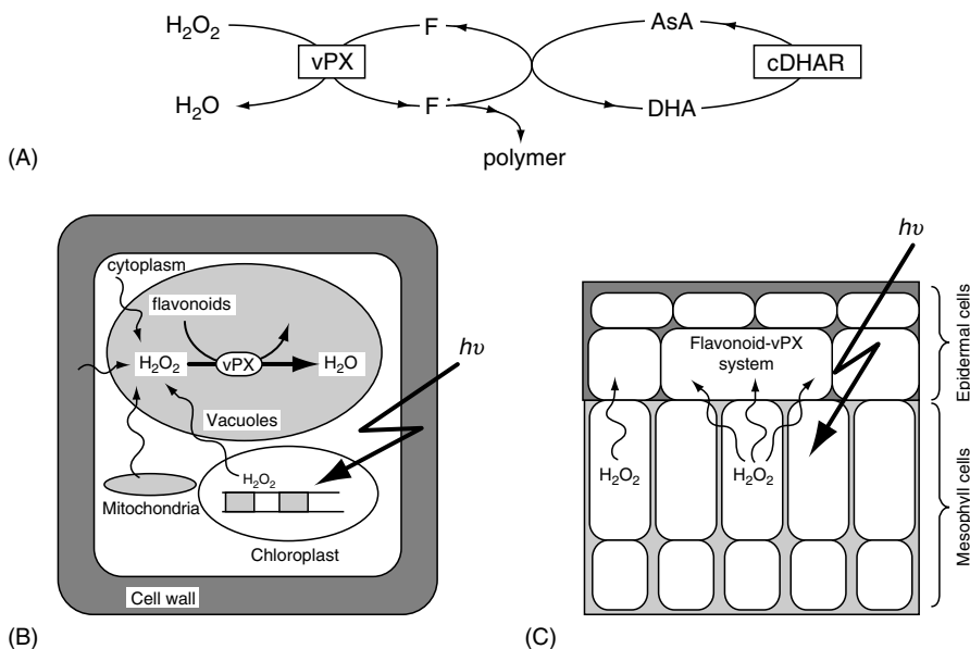
FIGURE 8.5 A proposed diagram for the protective function of flavonoids during stress (A). Scheme of the H_2O_2 -scavenging mechanism by flavonoids. vPX, vacuolar peroxidase; F, flavonoid; F', flavonoid radical; AsA, ascorbic acid; DHA, dehydroascorbic acid; h\nu , light energy; and cDHAR, cytosolic dehydroascorbic acid reductase. The diffusive nature of H_2O_2 enables vPX to scavenge it in vacuoles, even if the generating site is other than a vacuole (B). This concept can be expanded to cell-cell interaction. The photoproduced H_2O_2 may leak out from mesophyll cells and be scavenged in epidermal cells that have high flavonoid content (C). (Redrawn from Yamasaki, H., Sakihama, Y., and Ikehara, N., Plant Physiol. , 115, 1405, 1997. Copyright the American Society of Plant Biologists and reprinted with permission.)
