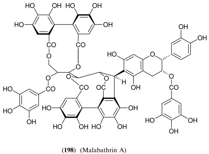
FIGURE 11.20 Structures of compounds 195–199.
