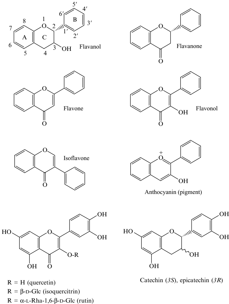
FIGURE 9.1 The main flavonoid classes and examples of common dietary flavonoids.
