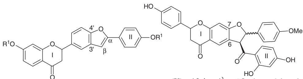
(78) R^1 = H , Lophirone I } — “Cleaved” chalcones — Lophira (79) R^1 = Me , Lophirone J } — lanceolata , rel. config., Ref. 48 (80) — Afzelone A } — C- \beta -epimers, Ochna afzelii , (81) Afzelone B } — rel. config., Ref.
