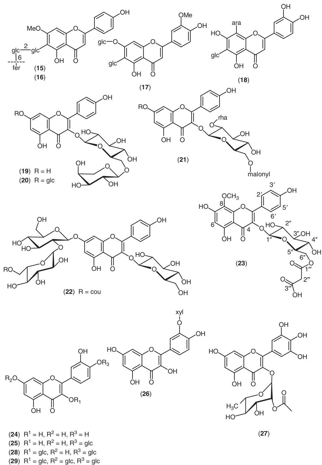
FIGURE 2.9 Structures of compounds 15–29. See Table 2.7 for names.
