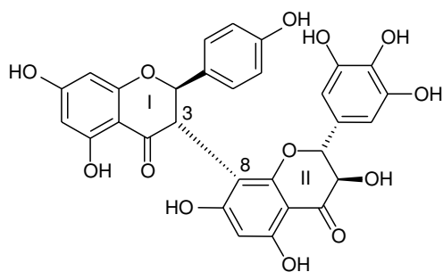
(96) GB-4, (I-2 R ,3 S ; II-2 R ,3 R ) } — Gnidia involucrata , (97) GB-4a, (I-2 S ,3 R ; II-2 R ,3 R ) } abs. config., Ref. 74
