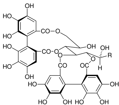
(214) R = 6-epicatechin (Camelliattannin C) (215) R = 8-epicatechin (Camelliattannin E)
