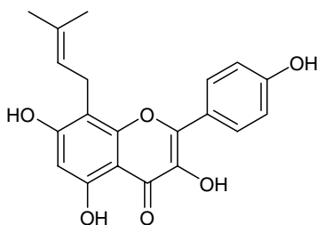
13.11
