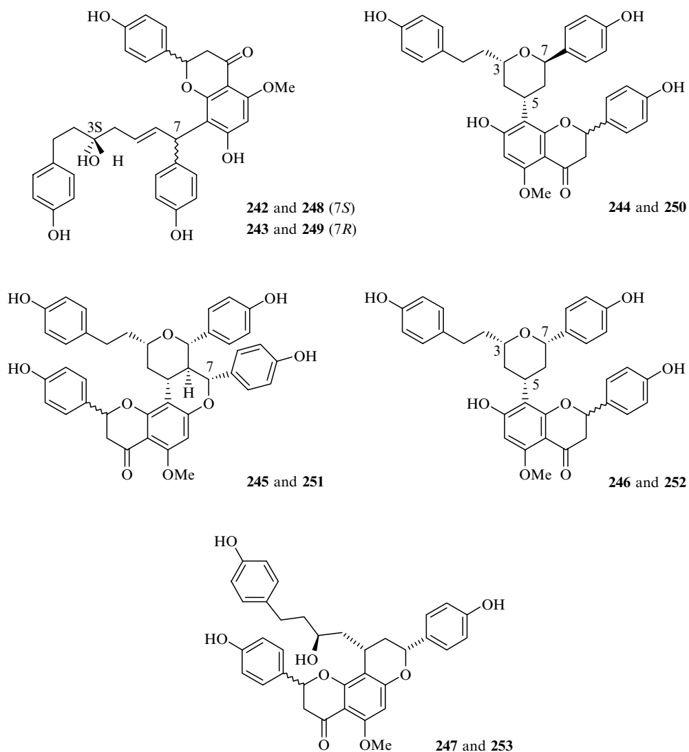
FIGURE 15.11 Diarylheptanoid flavanones.
