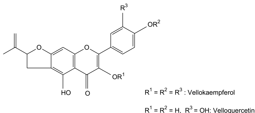
FIGURE 12.10 Furanoflavonols from Vellozia .
