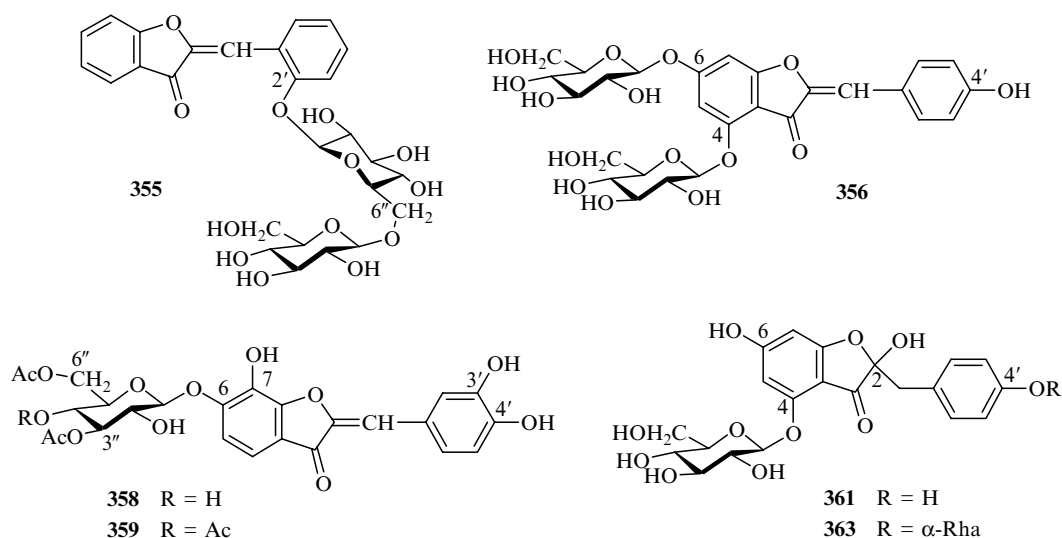
FIGURE 16.20 Aurone and auronol glycosides (see Table 16.14).
