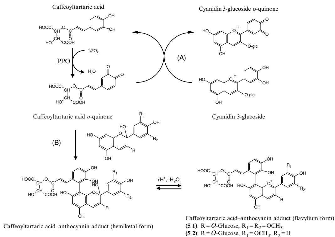
FIGURE 5.5 Anthocyanin reactions with caffeoyltartaric acid o -quinone coupled oxidation of cyanidin 3-glucoside (A) and nucleophilic addition of anthocyanins (B). Anthocyanin–caffeoyltartaric acid adducts are represented as one of the possible isomers, namely 2-(8-anthocyanin) caffeoyltartaric acid (5 1).
