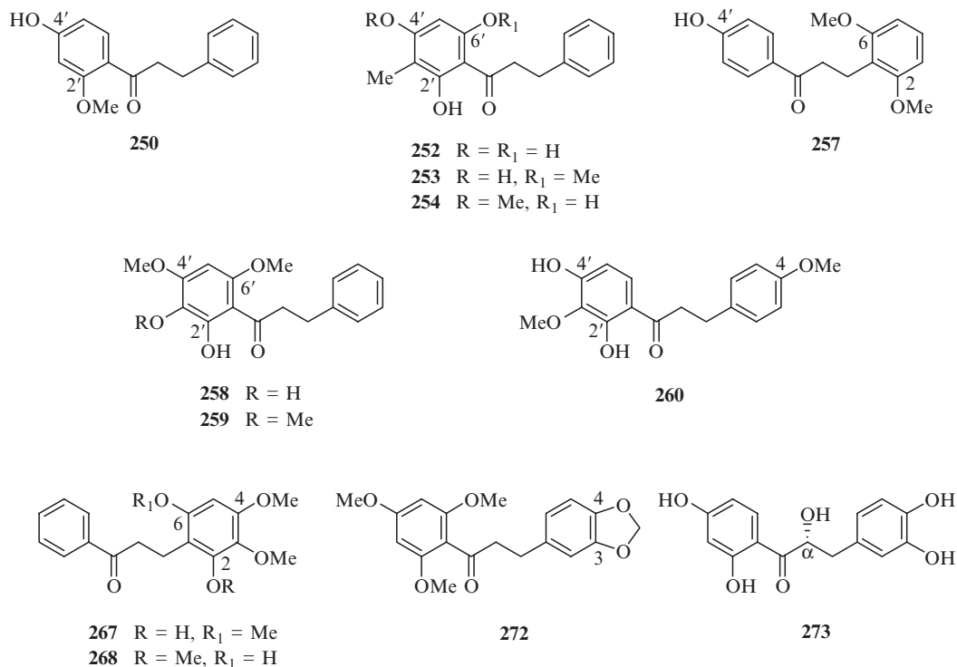
FIGURE 16.14 Dihydrochalcones with simple patterns of O -substitution (see Table 16.8).
