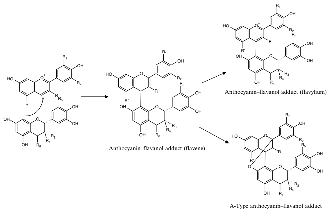
FIGURE 5.6 Postulated mechanism for formation of anthocyanin–flavanol adducts (flavanyl–anthocyanins). R, R', R 1 , R 2 as in Figure 5.1; R 3 = H, OH, galloyl; R 4 , R 5 = H, OH; R 6 = H, flavanyl.
