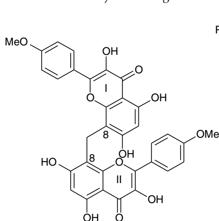
(140) Pentagrammetin — Pentagramma triangularis spp. triangularis , Ref. 41
