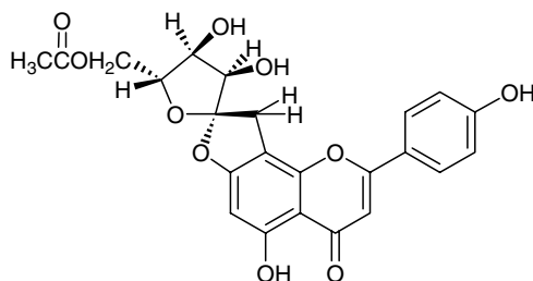
13.3
