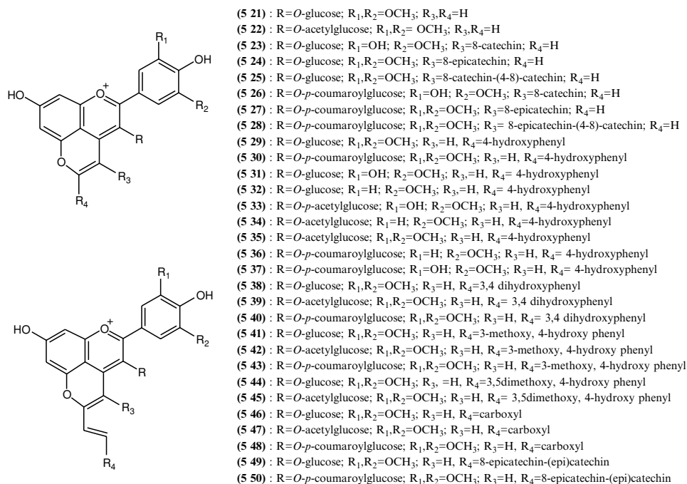
FIGURE 5.11 Structures of pyrananthocyanins.
