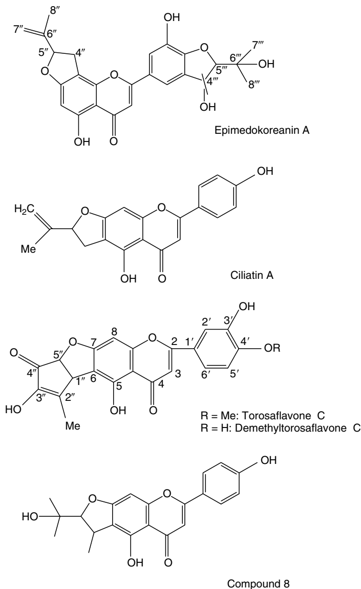
FIGURE 12.3 Furanoflavones.
