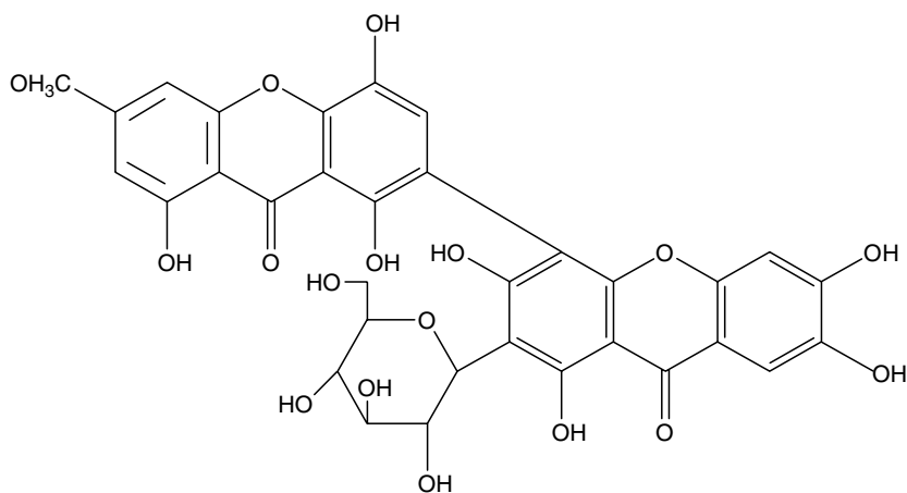
FIGURE 14.1 The structure of the flavone-xanthone dimer, swertifrancheside, isolated from Swertia franchetiana . (From Wang, J. et al., J. Nat. Prod. , 57, 211, 1994. With permission.)
