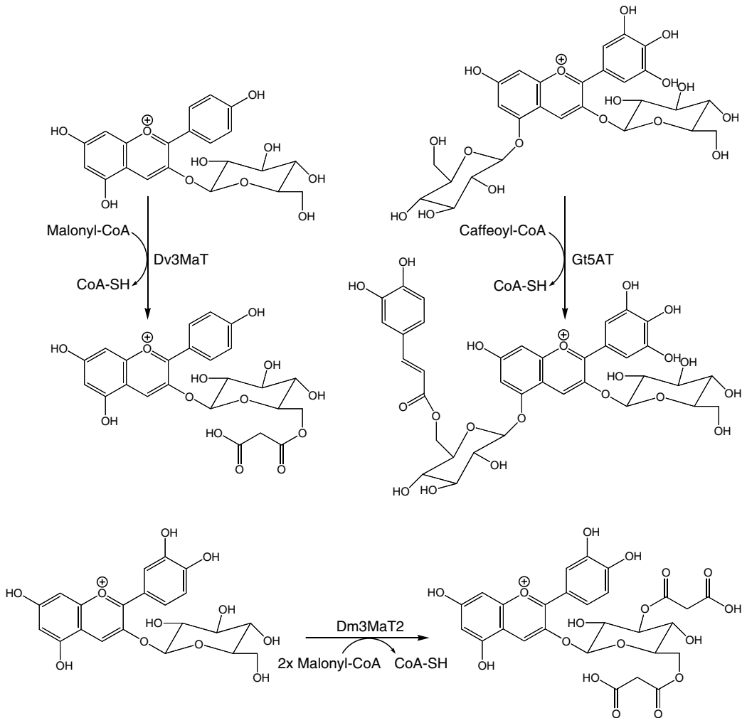
FIGURE 3.3 Examples of aliphatic and aromatic acylation of anthocyanins, as carried out by the malonyl-CoA:anthocyanidin 3- O -glucoside-6''- O -malonyltransferase (Dv3MaT from D. variabilis ), malonyl-CoA:anthocyanidin 3- O -glucoside-3'',6''- O -dimalonyltransferase (Dm3MaT2 from D. Xmorifolium ), and hydroxycinnamoyl-CoA:anthocyanin 5- O -glucoside-6''- O -hydroxycinnamoyltransferase (Gt5AT from G. triflora ).
