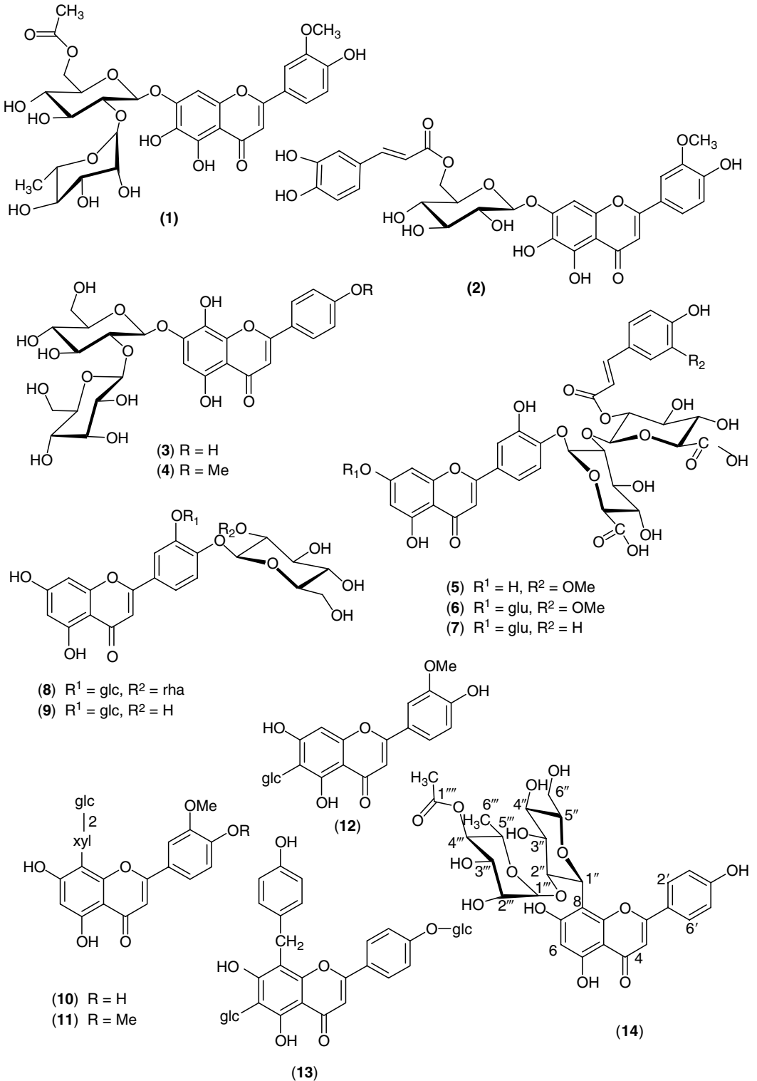
FIGURE 2.8 Structures of compounds 1–14. See Table 2.7 for names.
