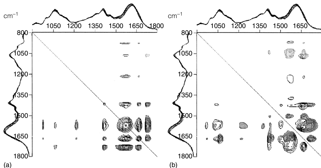
FIGURE 2.19 2D IR correlation spectra of the flavonoid-containing Chinese medicine “Qing Kai Ling.” (a) Synchronous IR spectrum; (b) asynchronous IR spectrum. In analogy to the corresponding 1D IR spectra, the units of the axis in both these 2D spectra are given in \text{cm}^{-1} . (Reprinted from Zuo, L. et al., J. Pharm. Biomed. Appl. , 30, 1491, 2003. Copyright 2003 Elsevier Science B.V. With permission.)
