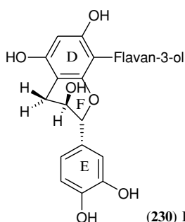
(230) E-conformer
