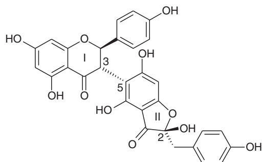
(74) Diastereoisomer shown } — Berchemia zeyheri , abs. config., Refs. 35, 36 (75) (II-2)- S -epimer
