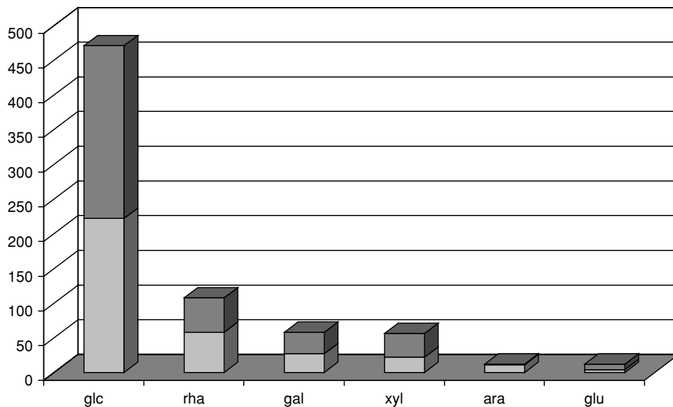
FIGURE 10.4 Numbers of anthocyanins containing the various monosaccharides identified in anthocyanins. The upper dark part of each bar represents the anthocyanins reported later than 1992. glc, glucose; rha, rhamnose; xyl, xylose; gal, galactose; ara, arabinose; glu, glucuronic acid. Some anthocyanins contain more than one type of monosaccharide.
