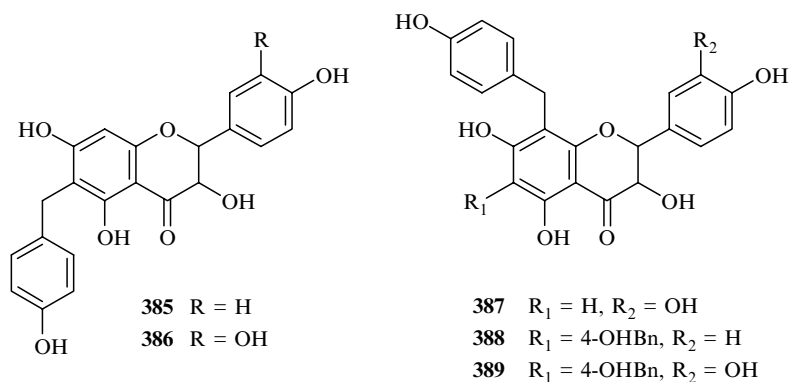
FIGURE 15.15 C-Benzyl-substituted dihydroflavonols (Bn, benzyl).
