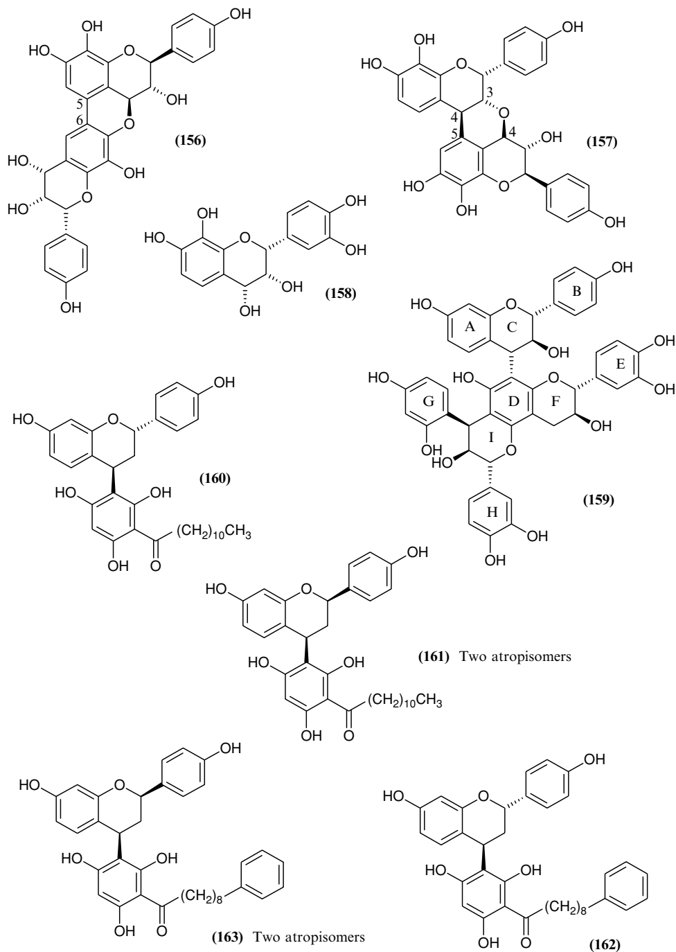
FIGURE 11.15 Structures of compounds 156–163 .
