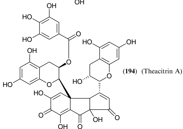
FIGURE 11.19 Structures of compounds 188–194.
