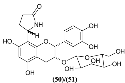
FIGURE 11.4 Structures of compounds 37–52.
