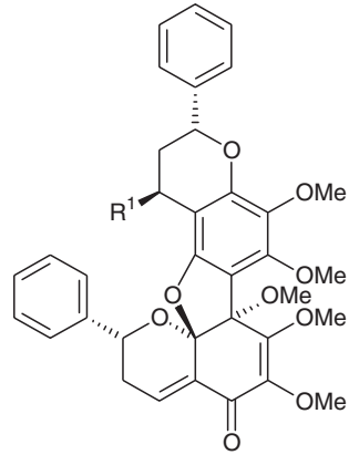
(130) R^1 = \text{OH} , Neocalycopteronone
