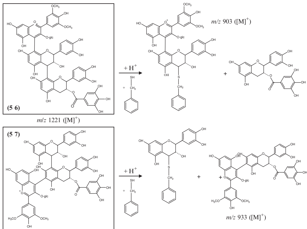
FIGURE 5.9 Hypothetical structures and thiolysis reaction of malvidin 3-glucoside–procyanidin B2 3'-gallate adducts.
