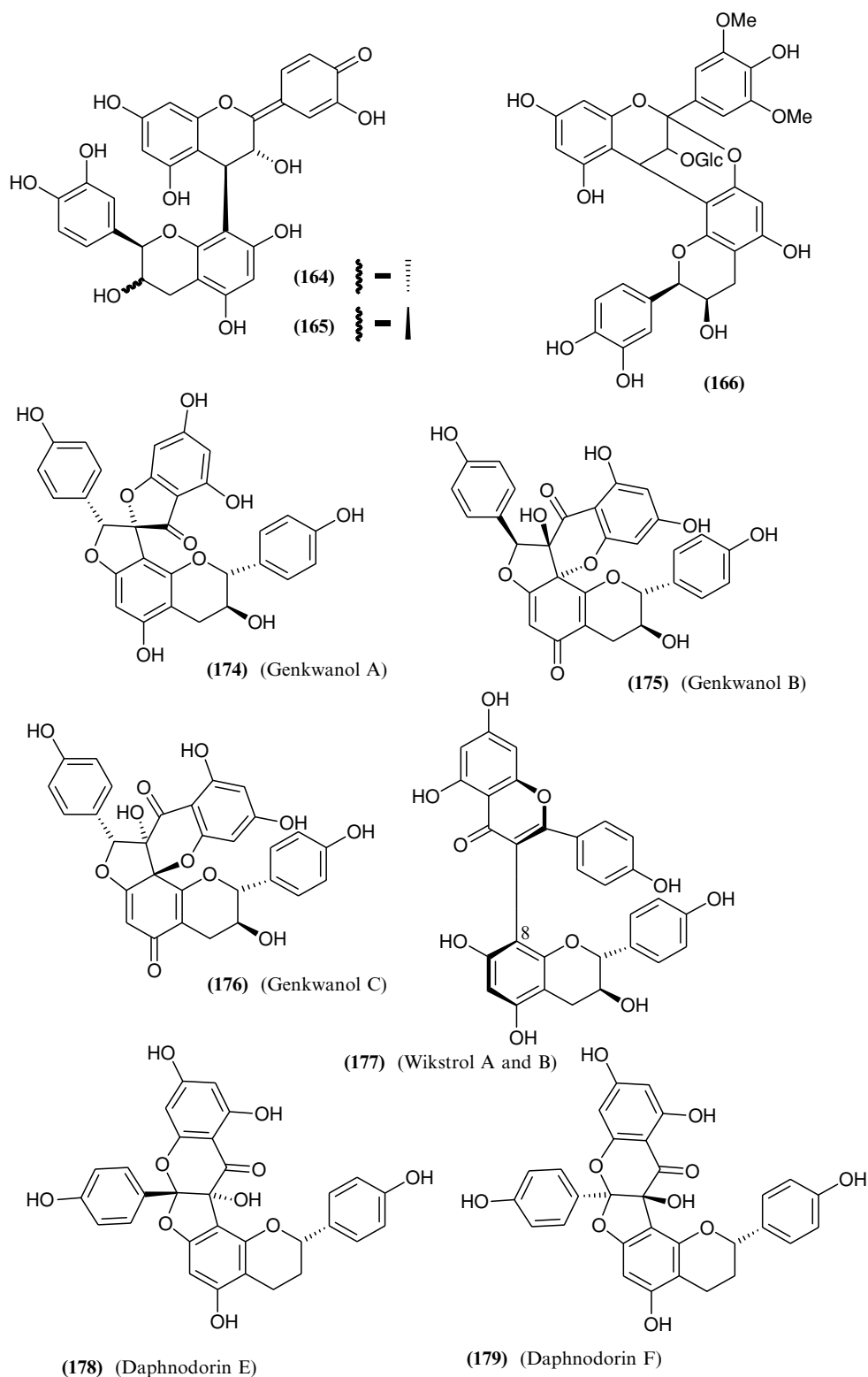
FIGURE 11.16 Structures of compounds 164–166 and 174–179.
