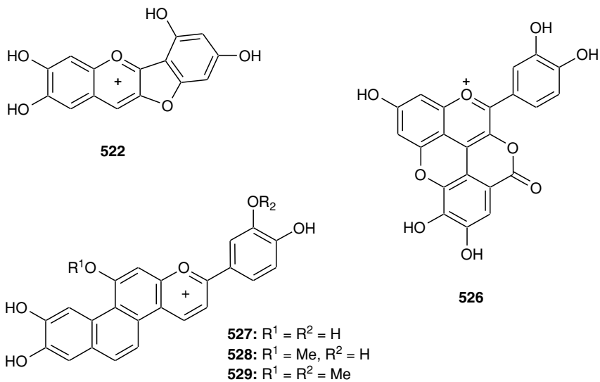
FIGURE 10.3 Some anthocyanidins with unusual structures; 522 , riccionidin A; 526 , rosacyanin B; 527–529 , sphagnorubins A–C.
