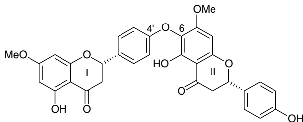
(98) I-7,II-7-Di-O-methyltetrahydrohinokiflavone — Cycas beddomei , abs. config., Ref. 80
