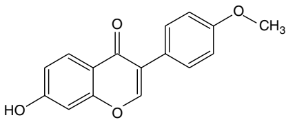
Formononetin
