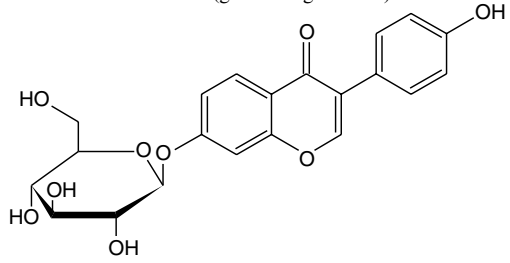
Daidzin (daidzein glucoside)
