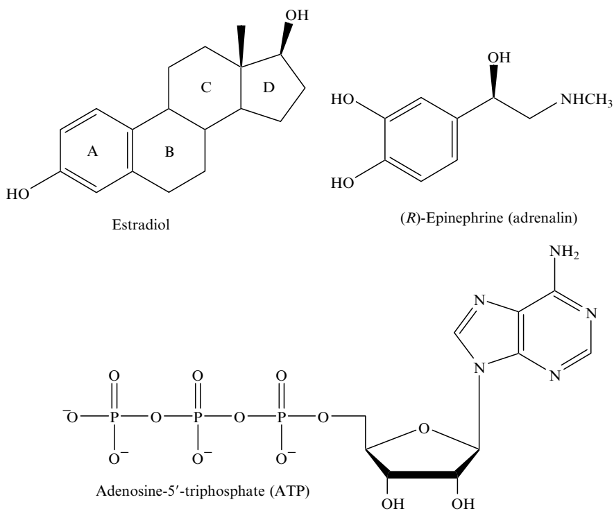
FIGURE 9.5 Structures of biologically important molecules with a formal structural resemblance to flavonoids.
