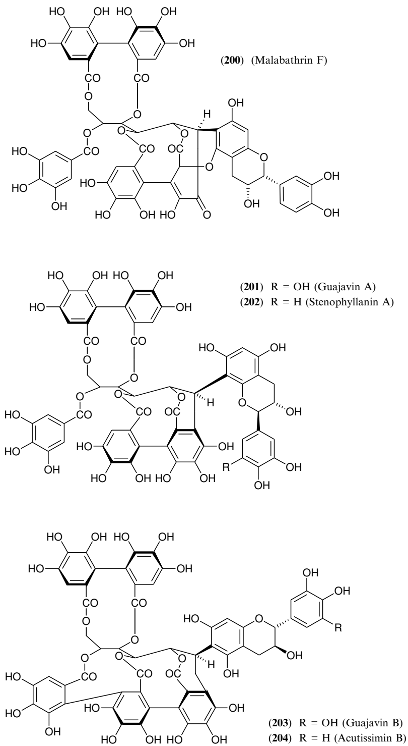
FIGURE 11.21 Structures of compounds 200–204.
