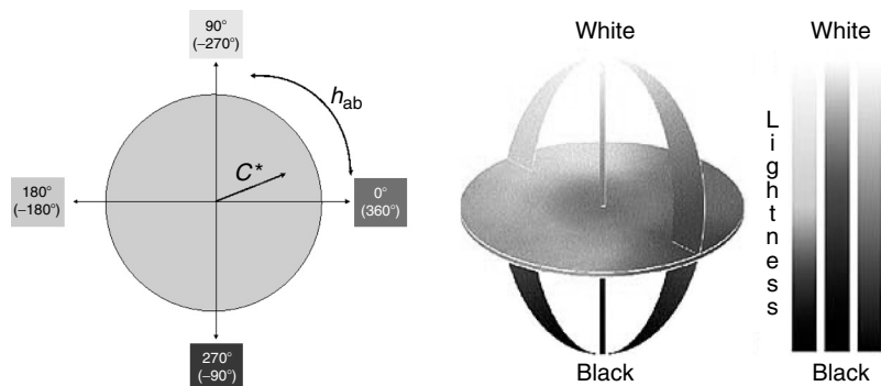
FIGURE 2.22 The three-dimensional CIELAB colour system. Left: h_{ab} (hue) describing the tonality of the color, where 0^\circ corresponds to red, 90^\circ corresponds to yellow, \pm 180^\circ corresponds to green, and 270^\circ (or -90^\circ ) corresponds to blue, C^* represents the chroma (or saturation), where 0 is a gray tone, while 100 is a pure hue. Right: the lightness ( L^* ) goes from black (0) to white (100).
