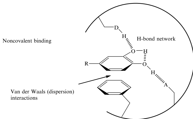
FIGURE 9.2 A schematic representation of molecular interactions at work in flavonoid–protein binding.
