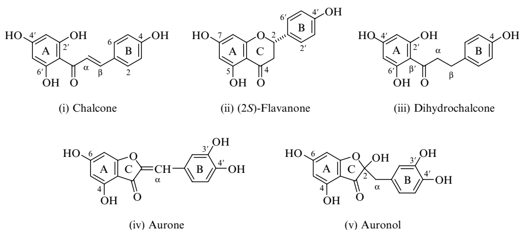
FIGURE 16.1 Guide to the structures, ring labeling, and atom numbering of chalcones, dihydrochalcones, aurones, and auronols. The corresponding flavanone structure is shown for reference.
