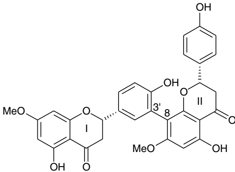
(12) (I-2S,II-2S)-I-7,II-7-Di-O-methyltetrahydroamentoflavone — Rhus retinorrhoea , abs. config., Ref. 23
