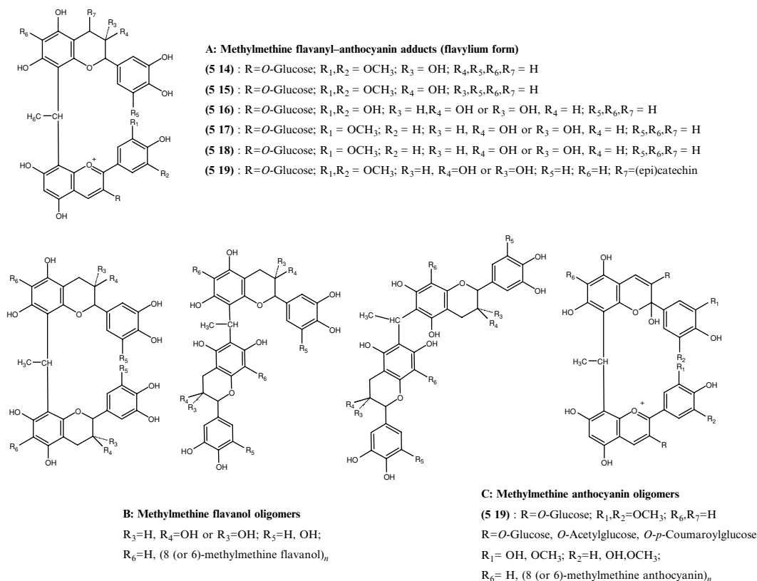
FIGURE 5.10 Structures of methylmethine-linked flavonoid derivatives.
