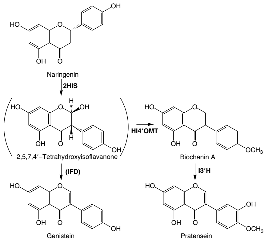
FIGURE 3.6 Biosynthetic route to isoflavones from the 5-hydroxyflavanone naringenin. Enzyme abbreviations are defined in the text.
