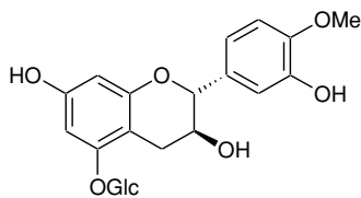
(76)
