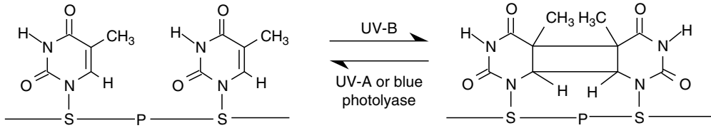
FIGURE 8.2 Formation of a thymine–thymine dimer by UV-B radiation, and repair by UV-A or blue light-activated photolyase.
