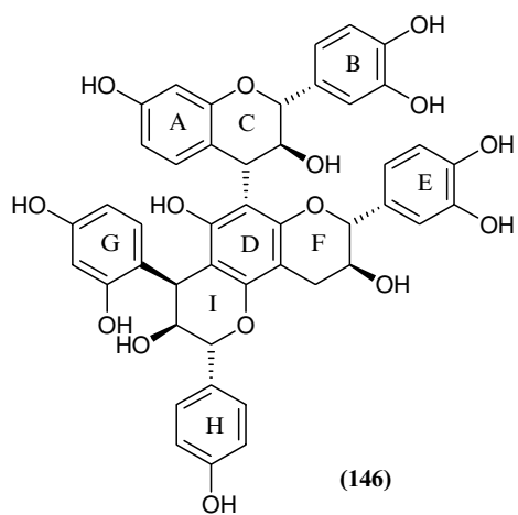
FIGURE 11.12 Structures of compounds 136–140 and 145–148.
