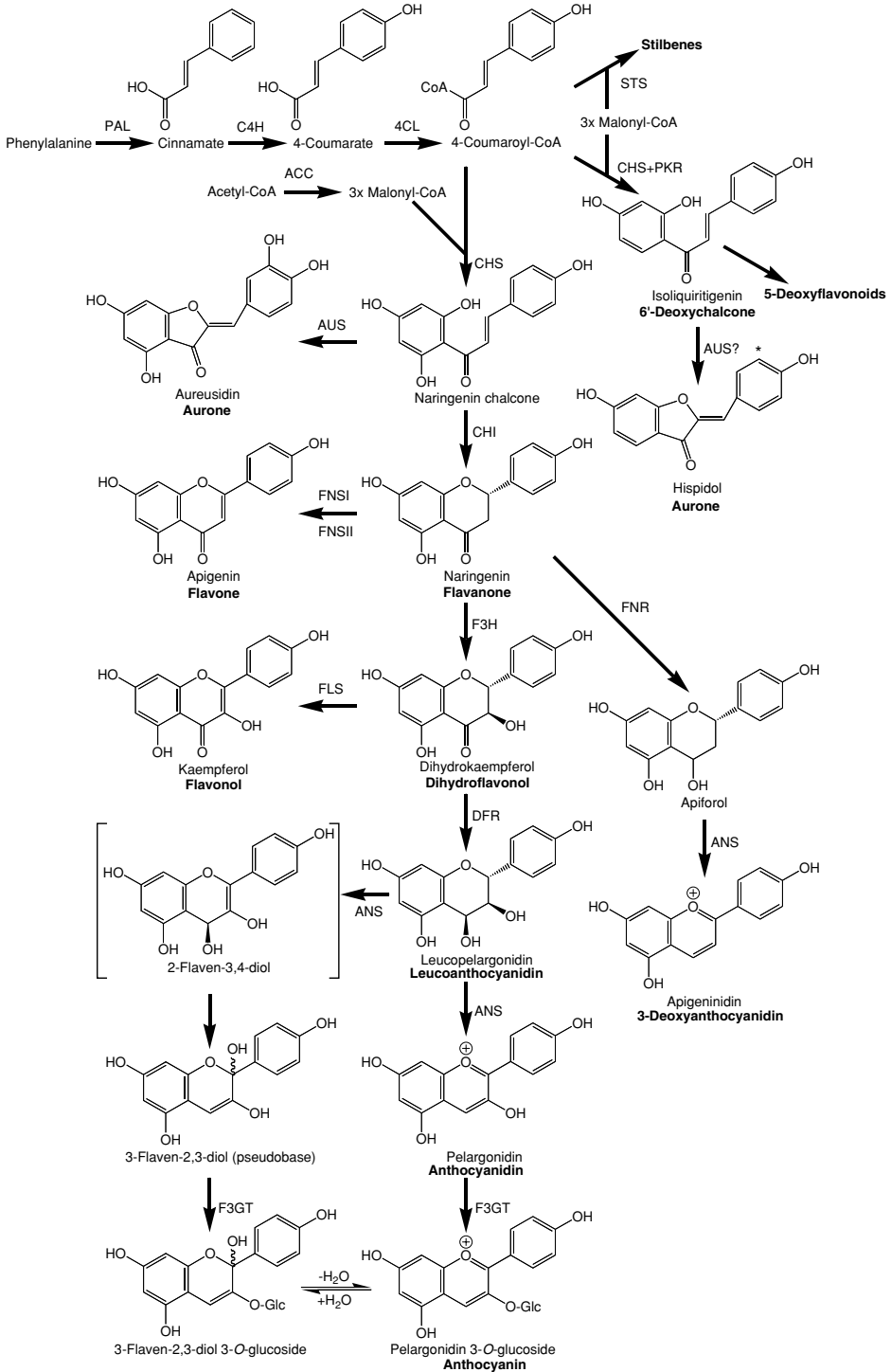
FIGURE 3.2 General phenylpropanoid and flavonoid biosynthetic pathways. The B-ring hydroxylation steps are not shown. For formation of anthocyanins from leucoanthocyanidins two routes are represented: a simplified scheme via the anthocyanidin (pelargonidin) and the likely in vivo route via the pseudobase. Enzyme abbreviations are defined in the text and in Table 3.1.
