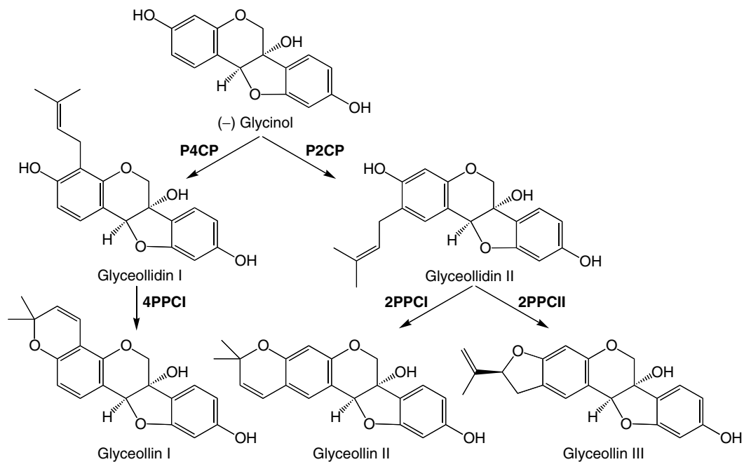
FIGURE 3.7 Biosynthetic route to complex glyceollin phytoalexins from glycinol. Enzyme abbreviations are P2CP, pterocarpan 2-C-prenyltransferase; P4CP, pterocarpan 4-C-prenyltransferase; 2PPCI/2PPCII, prenylpterocarpan cyclases acting at the C-2 prenyl group; 4PPCI, prenylpterocarpan cyclase acting at the C-4 prenyl group.
