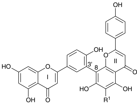
(12) (I-2S,II-2S)-I-7,II-7-Di-O-methyltetrahydroamentoflavone — Rhus retinorrhoea , abs. config., Ref. 23
