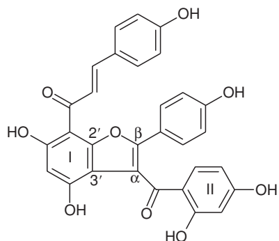
(28) Calodenin A — Ochna calodendron , Ref. 32
