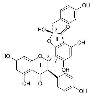
(100) Diastereoisomer shown } — Berchemia zeyheri , abs. (101) (II-2)- S -epimer } config., Refs. 35, 36
