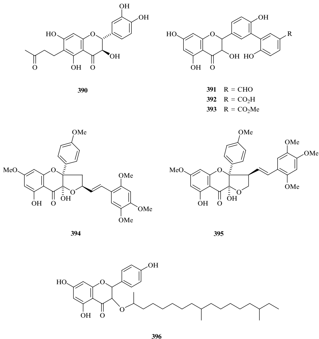
FIGURE 15.16 Dihydroflavonols with miscellaneous substituents.
