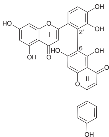
(46) 3''-Desoxydicranolomin } — Plagiommium undulatum , Ref. 85 (47) I-2,3-Dihydro derivative }
