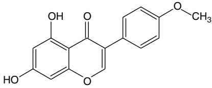
Biochanin A
