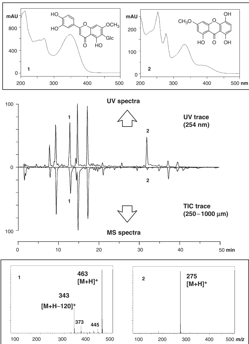
FIGURE 1.8 LC–UV–MS analysis of a methanolic extract of Gentianella cabrerana . The UV trace was recorded at 254 nm and the UV spectra from 200 to 500 nm. The LC–TSP–MS trace was recorded from 250 to 1000 μm. HPLC: Column Novapak C 18 (150 × 3.9 mm, 4 μm); gradient of CH 3 CN–H 2 O (containing 0.1% TFA) 5:95 → 65:35 in 50 min; flow-rate 1 ml/min; 0.5 M NH 4 OAc (0.2 ml/min) postcolumn. TSP: positive ion mode; filament off; vaporiser 100°C; source 280°C. (From Hostettmann, K., Wolfender, J.L., and Rodriguez, S., Planta Med. , 63, 2, 1997. With permission.)
