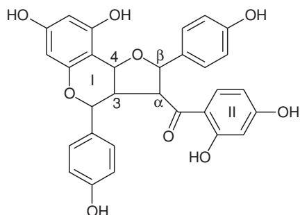
(26) Cordigol — Cordia goetzei , no config. indicated, Ref. 31
