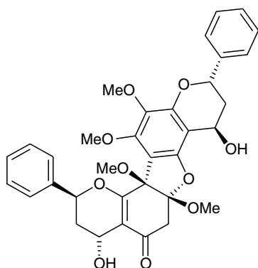
(135) Calyflorenone D — Calycopteris floribunda , abs. config., Ref. 104
