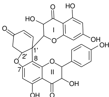
(146) Hypnumbiflavonoid A — Hypnum cupressiforme , rel. config., Ref. 34 See also the structures of two phenylacetic acid-substituted aromadendrin analogs from the same source.
