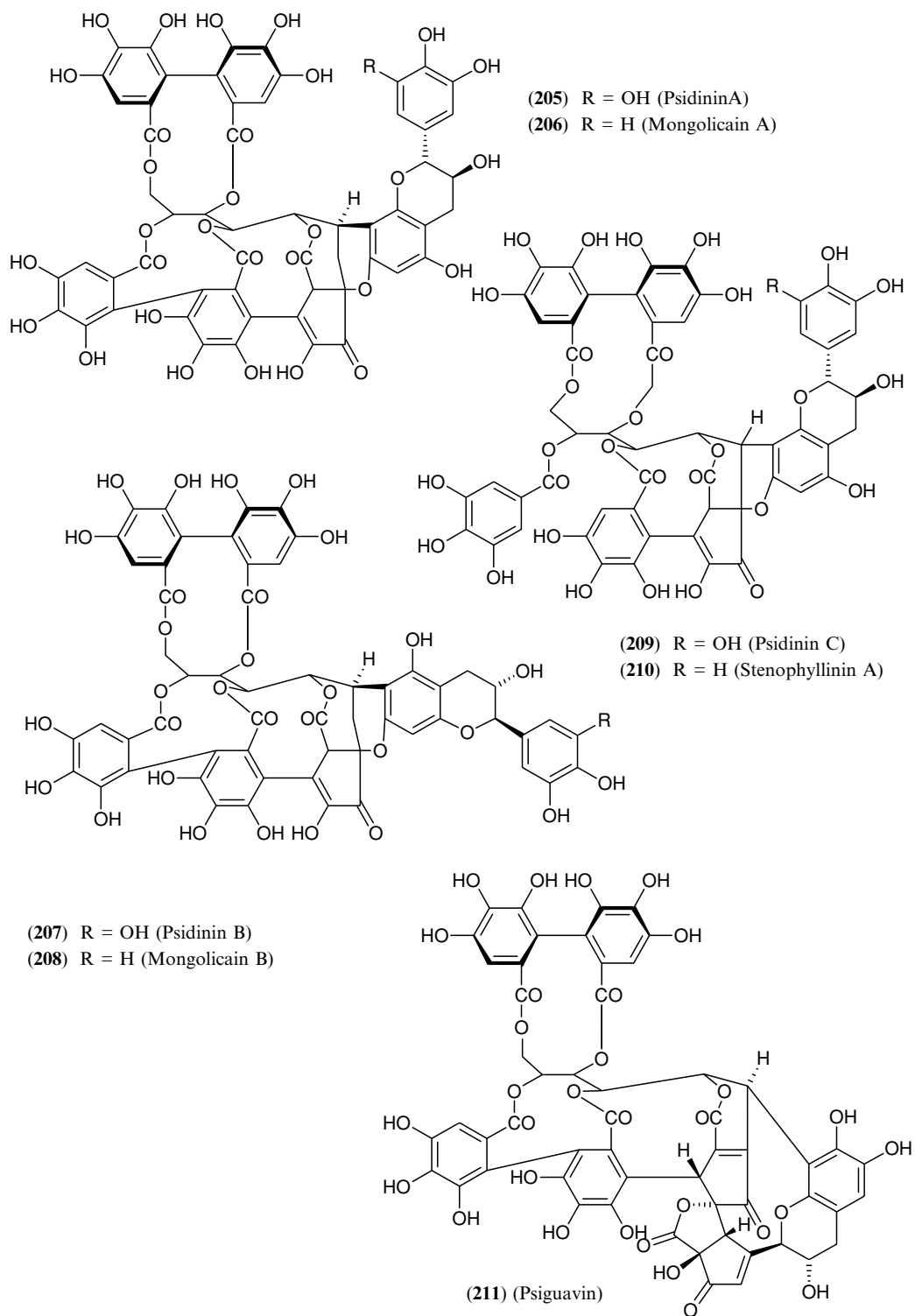
FIGURE 11.22 Structures of compounds 205–211.
