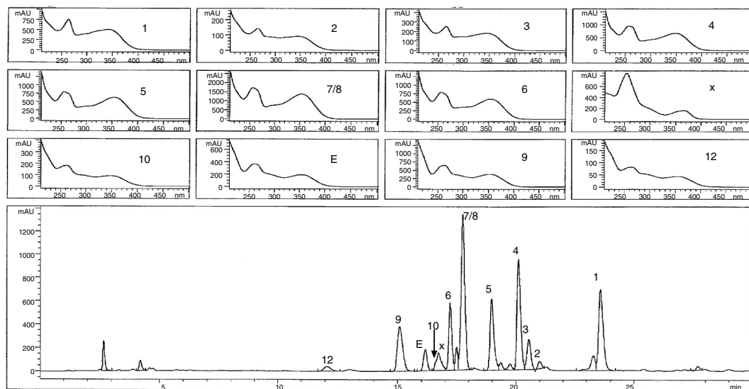
FIGURE 1.6 LC-UV chromatogram of a methanolic extract of the aerial parts of Epilobium angustifolium enriched by n -BuOH-H 2 O partition. Column Novapak C 18 (150 × 3.9 mm, 4 μm); step gradient of CH 3 CN-H 2 O (containing 0.05% TFA): 0 min 10% CH 3 CN, 4 min 12%, 12 min 12%, 16 min 18%, 30 min 25%; flow-rate 1 ml/min; chromatogram recorded at 350 nm. (From Ducrey, B., Wolfender, J.L., Marston, A., and Hostettmann, K., Phytochemistry , 38, 129, 1995. With permission.)
