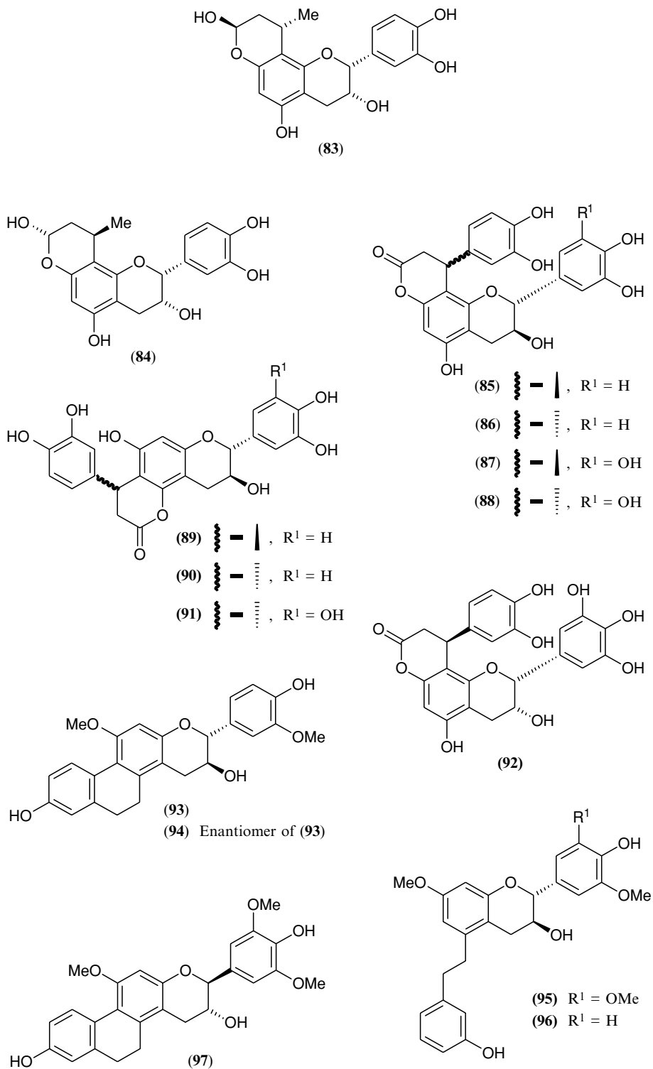
FIGURE 11.8 Structures of compounds 82–97.
