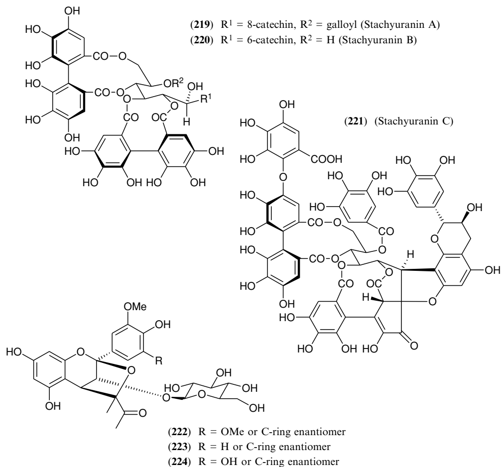
FIGURE 11.25 Structures of compounds 219–224.
