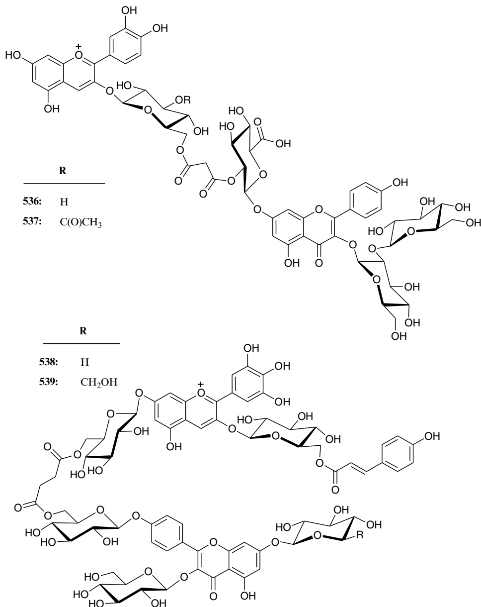
FIGURE 10.9 (6''-(cyanidin 3-glucosyl)) (2'''-(kaempferol 3-[2''-(glucosyl)(glucoside)]-7-glucuronosyl)-malonate ( 536 ) and (6''-(cyanidin 3-[3''-(acetyl)glucosyl]) (2'''-(kaempferol 3-[2''-(glucosyl)(glucoside)]-7-glucuronosyl))malonate ( 537 ) isolated from pale-purple flowers of chive ( Allium schoenoprasum ), 11 and (6'''-(delphinidin 3-[6''-( p -coumaryl)glucoside]-7-glucosyl)) (6''''-(kaempferol 3-glucoside-7-xyloside-4'-glucosyl)succinate ( 538 ) and (6'''-(delphinidin 3-[6''-( p -coumaryl)glucoside]-7-glucosyl)) (6''''-(kaempferol 3-glucoside-7-glucoside-4'-glucosyl)succinate ( 539 ) from blue Agapanthus flowers. 12
