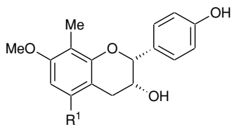
(74) R^1 = \text{H}
