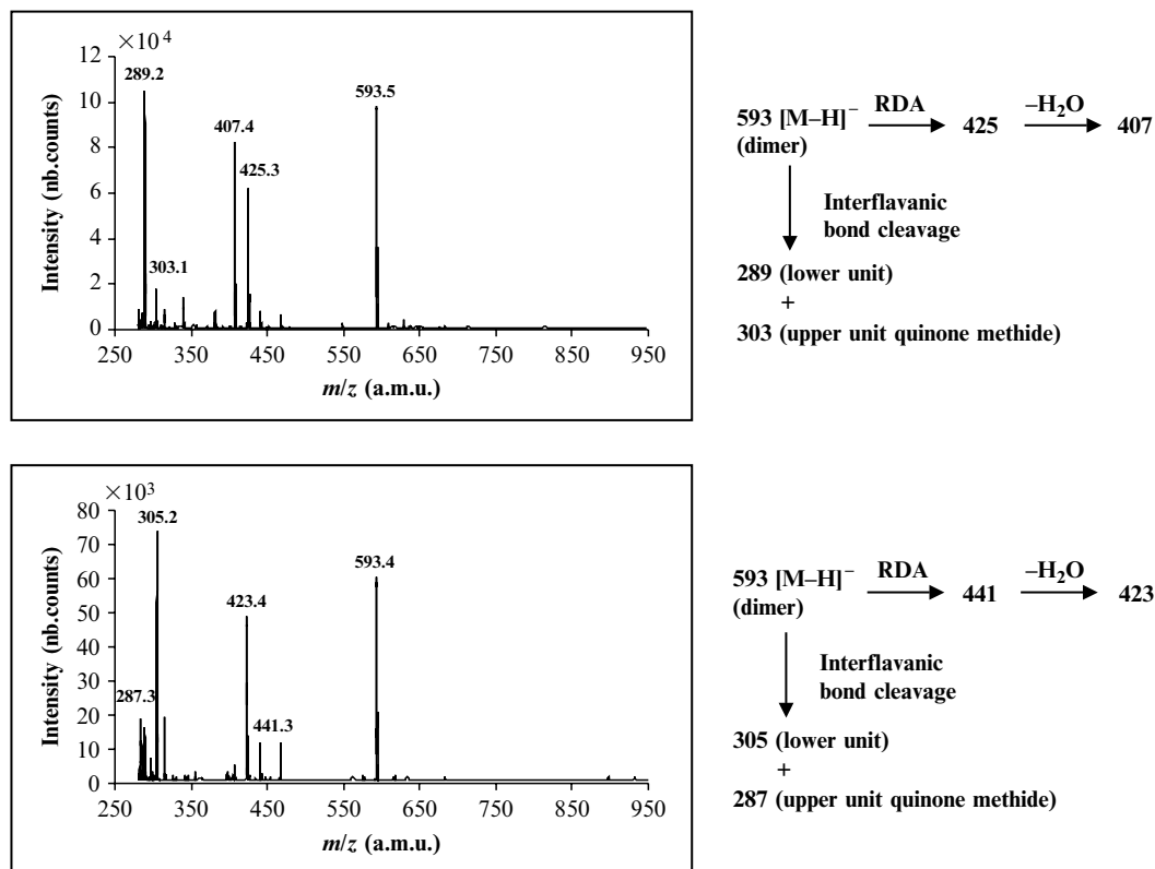
FIGURE 5.3 ESI-Q mass spectra obtained from two proanthocyanidin dimers.
