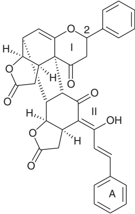
(123) Chalcocaryanone A (I-2R)
