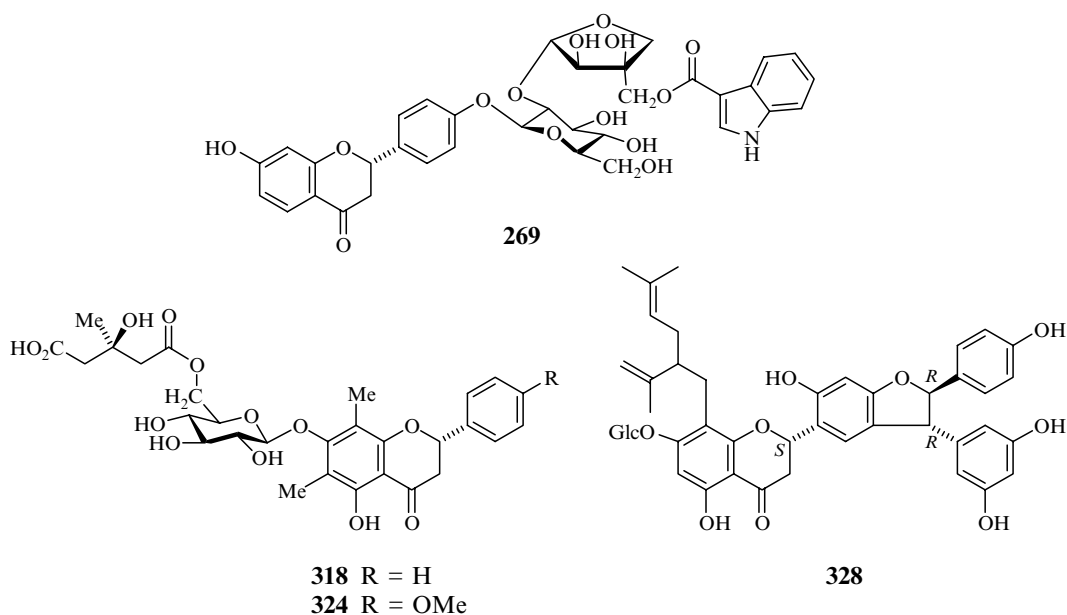
FIGURE 15.13 Examples of flavanone glycosides.
