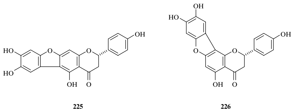
FIGURE 15.8 Anastatins.
