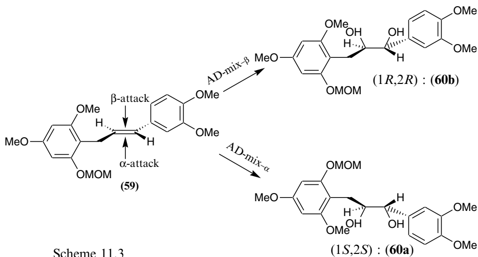
Scheme 11.3
