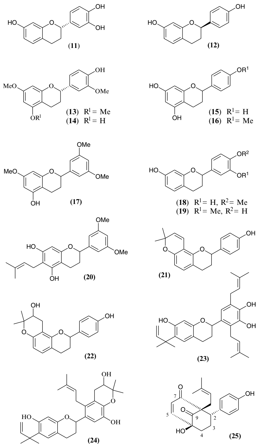
FIGURE 11.2 Structures of compounds 11–25.
