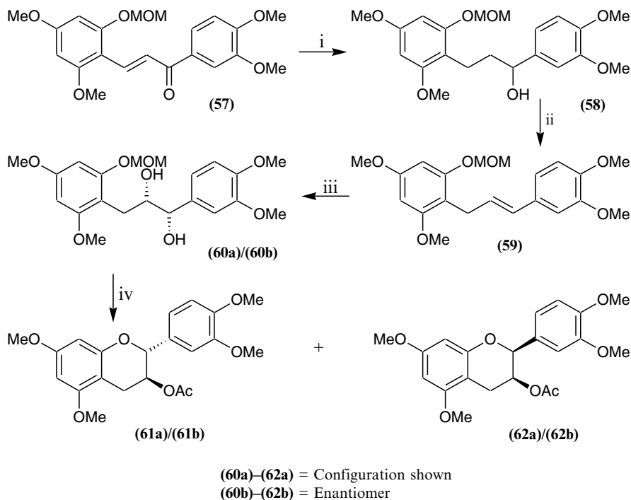
Scheme 11.2
