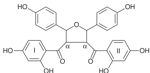
(25) Cordigone — Cordia goetzei , no config. indicated, Ref. 31
