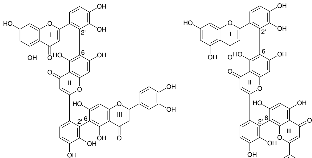
(152) Distichumtrilineol — Rhizogonium distichum , Ref. 86
