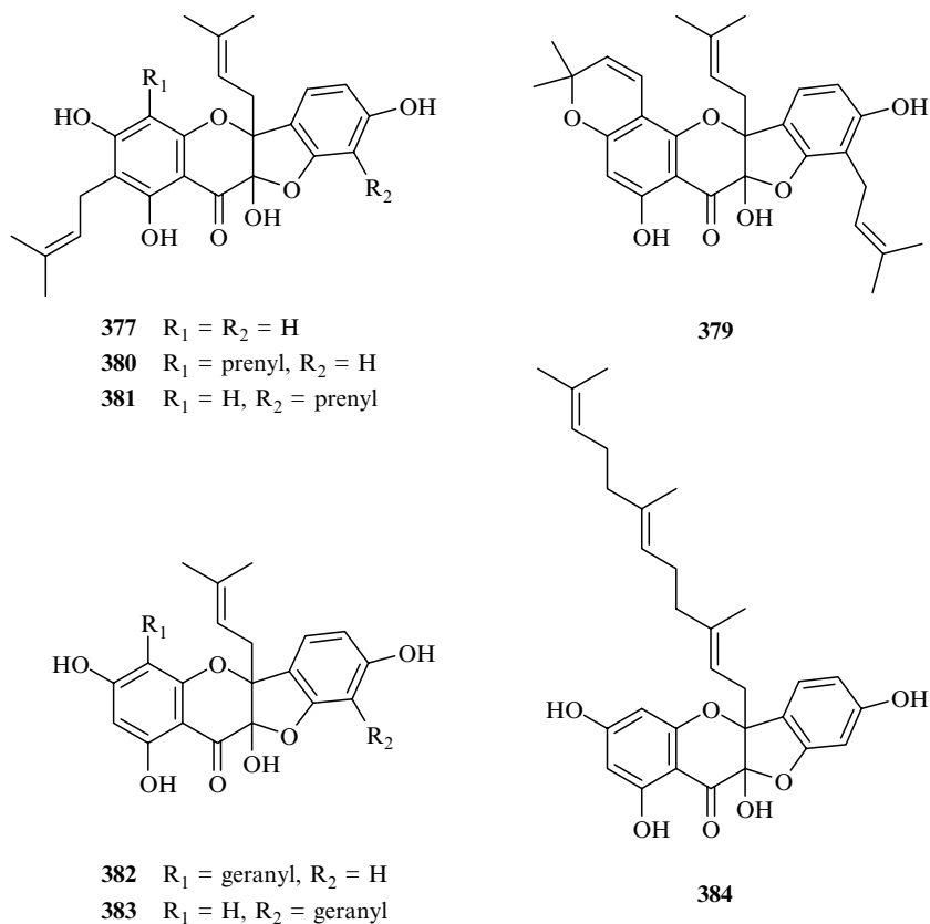
FIGURE 15.14 C-2-Isoprenylated C-3–C-2'-ether-linked dihydroflavonols.
