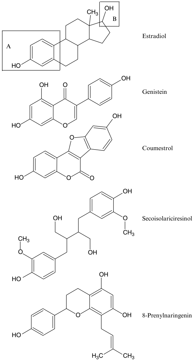
FIGURE 7.1 The structural relationship between phytoestrogens and 17\beta -estradiol.
