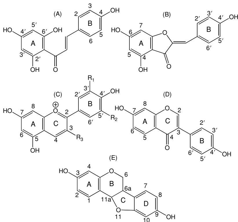
FIGURE 3.1 Base structures of a chalcone (A), an aurone (B), the main anthocyanidins (C), an isoflavonoid (D), and a pterocarpin (E). The lettering of the carbon rings is shown, as well as the numbering of the key carbons. Note that the numbering is different for each type of compound. For the majority of flavonoid types the numbering is as for the anthocyanidins, and for the cinnamic acids it is as for the chalcones. R_1 , R_2 , and R_3 substitutions determine the various common anthocyanidins. The common 3-hydroxyanthocyanidins ( R_3 = \text{OH} ) are pelargonidin ( R_1 and R_2 = \text{H} ), cyanidin ( R_1 = \text{OH} and R_2 = \text{H} ), delphinidin ( R_1 and R_2 = \text{OH} ), peonidin ( R_1 = \text{OCH}_3 and R_2 = \text{H} ), petunidin ( R_1 = \text{OCH}_3 and R_2 = \text{OH} ), and malvidin ( R_1 and R_2 = \text{OCH}_3 ). The rare 3-deoxyanthocyanidins ( R_3 = \text{H} ) are apigeninidin ( R_1 and R_2 = \text{H} ), luteolinidin ( R_1 = \text{OH} and R_2 = \text{H} ), and tricetinidin ( R_1 and R_2 = \text{OH} ).
