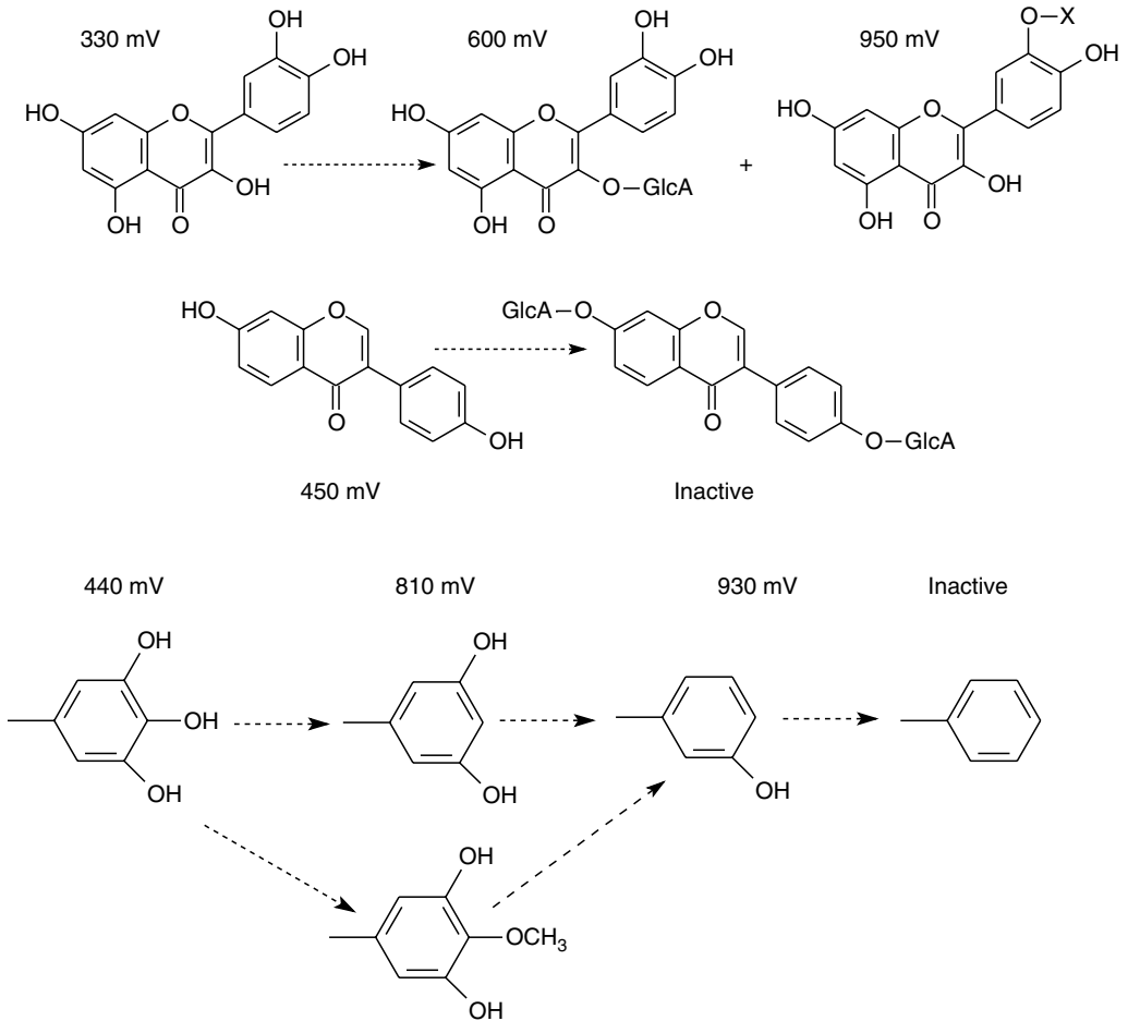
FIGURE 6.1 Illustration of the effects of mammalian metabolism and microbial metabolism on the redox potential of (poly)phenols found in plasma compared with their precursors in the diet and the aglycones commonly used in studies in vitro . (Reprinted from Clifford, M.N., Planta Med. , 12, 1103, 2004. With permission.)
