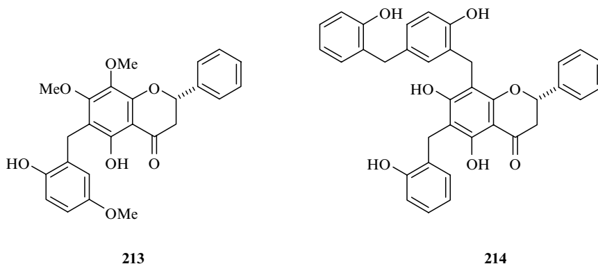
FIGURE 15.6 C-Benzyl-substituted flavanones.
