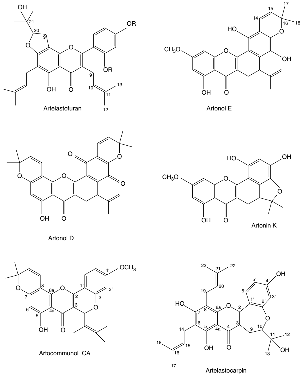
FIGURE 12.6 Flavones from Artocarpus spp.
