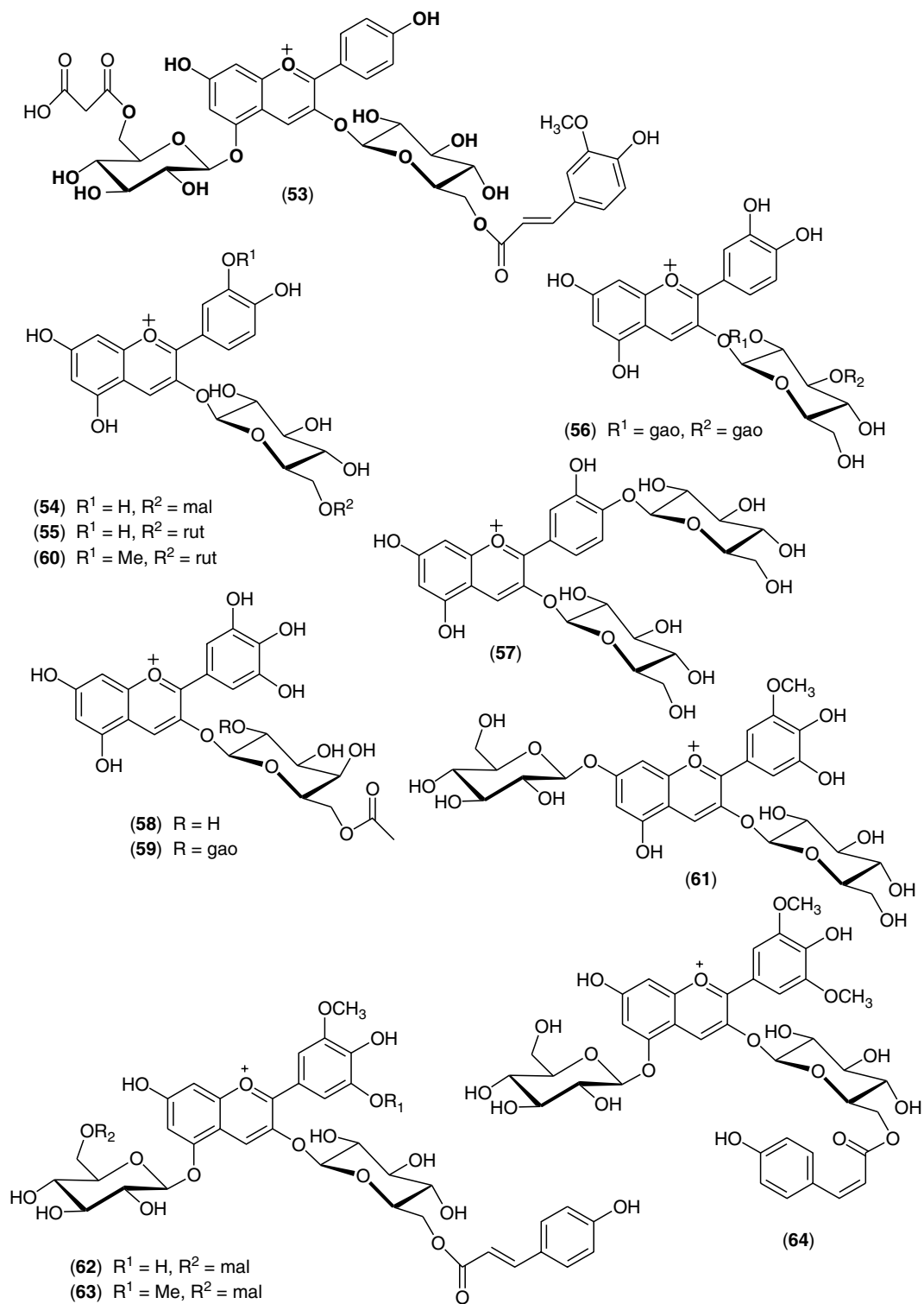
FIGURE 2.12 Structures of compounds 53–64. See Table 2.7 for names.
