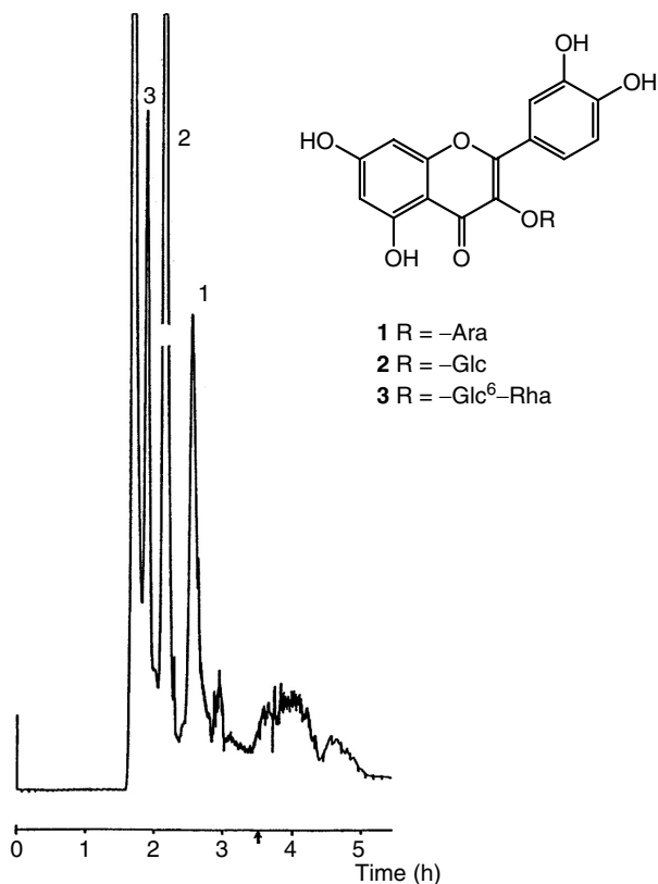
FIGURE 1.1 Separation of flavonol glycosides from Tephrosia vogelii (Leguminosae) with a Quattro CPC instrument. Solvent system, \text{CHCl}_3 -MeOH-EtOH- \text{H}_2\text{O} (5:3:3:4); mobile phase, upper phase; flow-rate, 3 ml/min; detection, 254 nm; sample, 500 mg MeOH extract. (From Sutherland, I.A., Brown, L., Forbes, S., Games, G., Hawes, D., Hostettmann, K., McKerrell, E.H., Marston, A., Wheatley, D., and Wood, P., J. Liq. Chrom. Relat. Technol. , 21, 279, 1998. With permission.)
