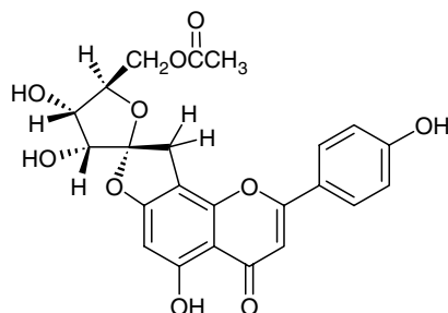
13.4
