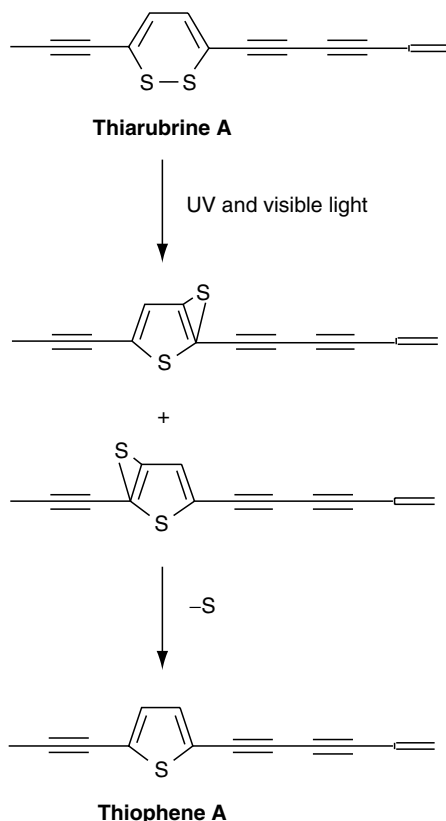
FIGURE 8.1 Conversion of the antimicrobial agent, thiarubrine A, to its photoproduct, thiophene A, by exposure to ultraviolet and visible radiation. (Redrawn from Page, J.E. and Towers, G.H.N., Planta , 215, 478, 2002. With permission.)
