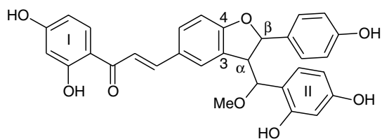
(41) Azobebechalcone — Lophira alata , rel. config., Ref. 50
