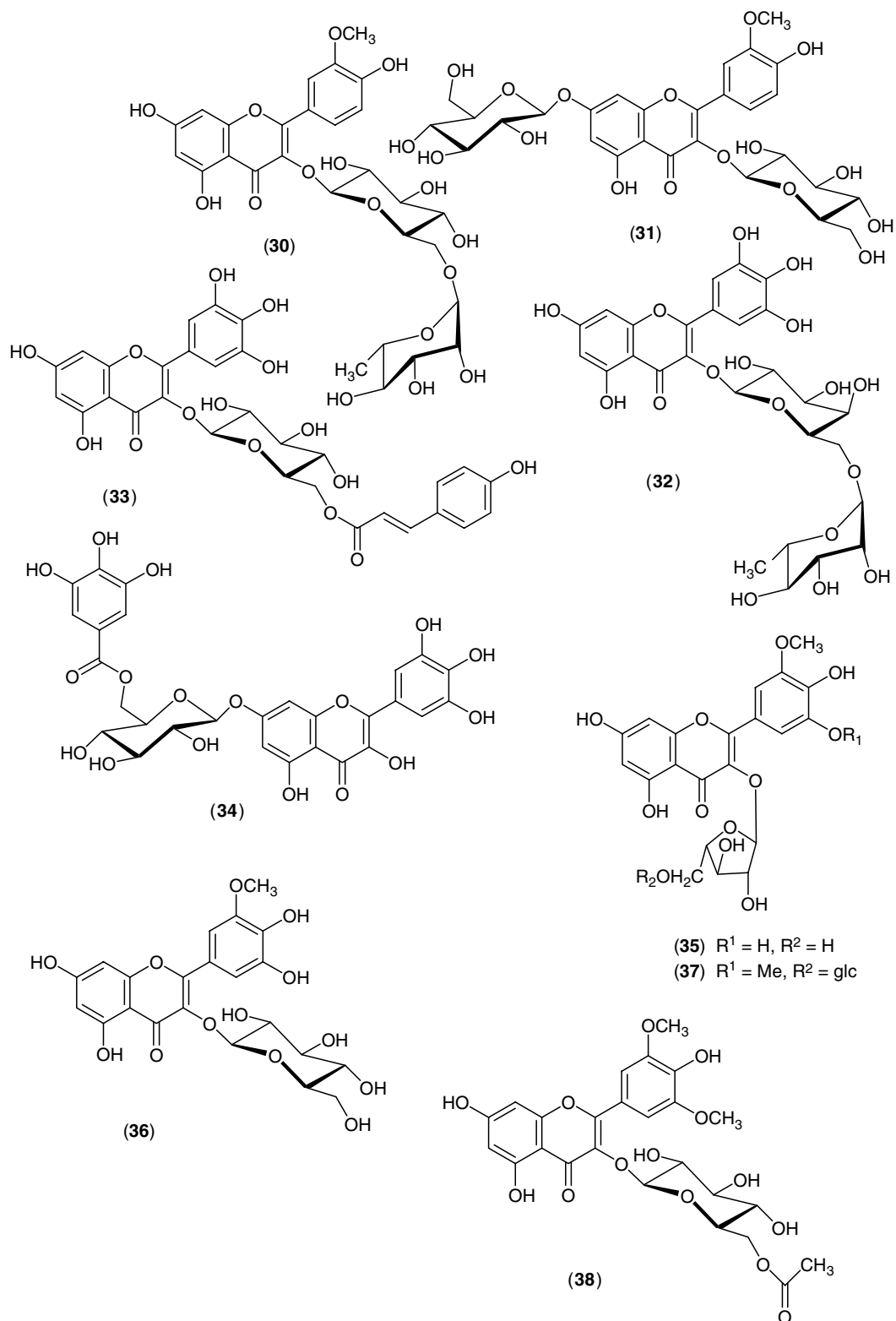
FIGURE 2.10 Structures of compounds 30–38. See Table 2.7 for names.
