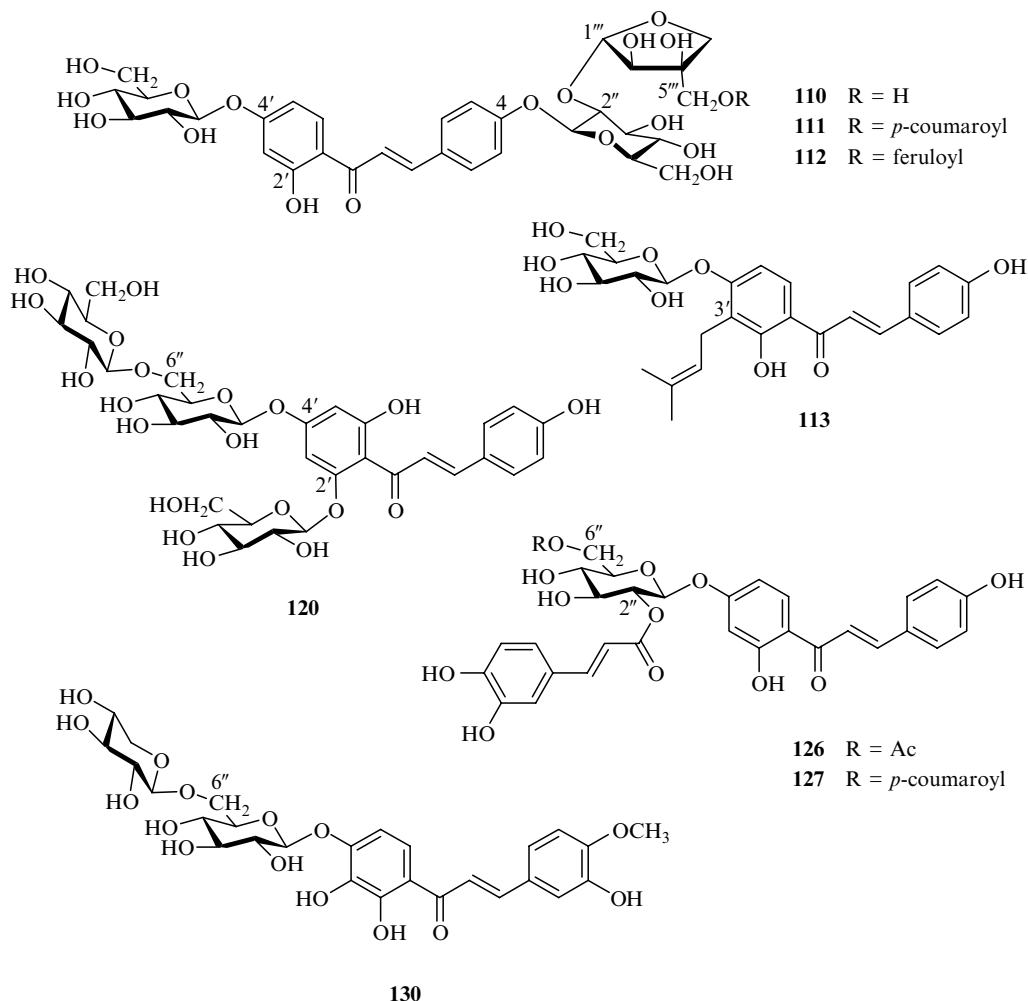
FIGURE 16.8 Chalcone glycosides (see Table 16.3).
