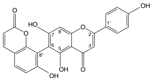
6-(8''-Umbelliferyl)-apigenin
