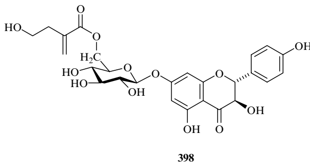
FIGURE 15.17 Acylated dihydroflavonol glycoside.
