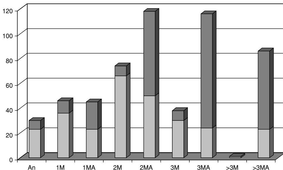
FIGURE 10.1 Anthocyanidins (An) and anthocyanins grouped according to their content of monosaccharide units and acylation. The vertical axis represents the number of pigments. The upper dark part of each bar represents the anthocyanins reported later than 1992. 1M, one monosaccharide unit; 1MA, one monosaccharide unit plus acylation; 2M, two monosaccharide units; 2MA, two monosaccharide units plus acylation; 3M, three monosaccharide units; 3MA, three monosaccharide units plus acylation; >3M, more than three monosaccharide units; >3MA, more than three monosaccharide units plus acylation.
