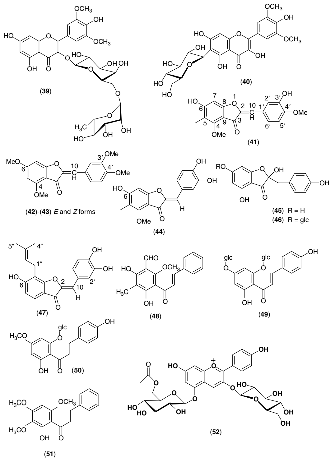
FIGURE 2.11 Structures of compounds 39–52. See Table 2.7 for names.
