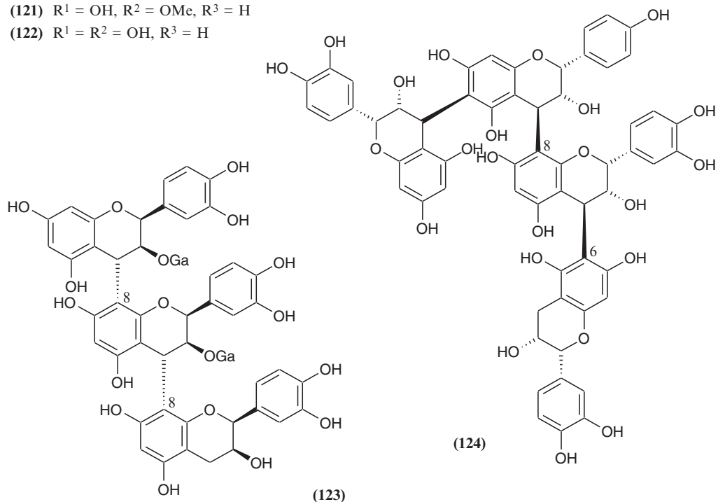
FIGURE 11.10 Structures of compounds 114–118 and 120–124.
