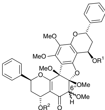
(136) R^1 = R^2 = H , 6'' \beta -OMe, Calyflorenone C (137) R^1 = H , R^2 = Me , 6'' \alpha -OMe, 6- epi -Calyflorenone B (138) R^1 = R^2 = H , 6'' \alpha -OMe, 6- epi -Calyflorenone C Calycopteris floribunda , abs. config., Ref. 104
