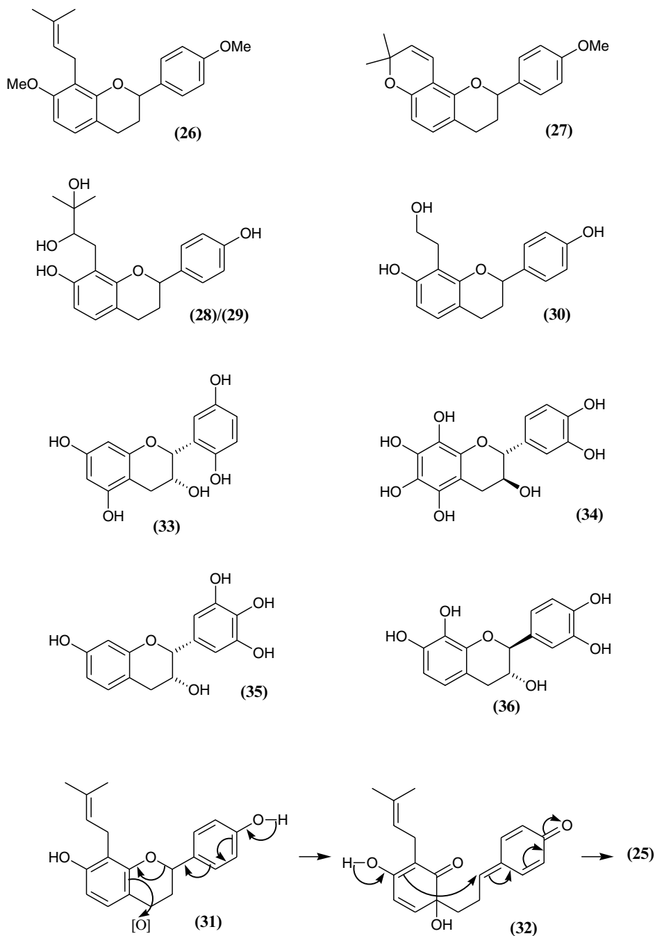
FIGURE 11.3 Structures of compounds 26–36 including Scheme 11.1: Proposed biogenetic conversion of brosimine B (31) into acutifolin A (25).
