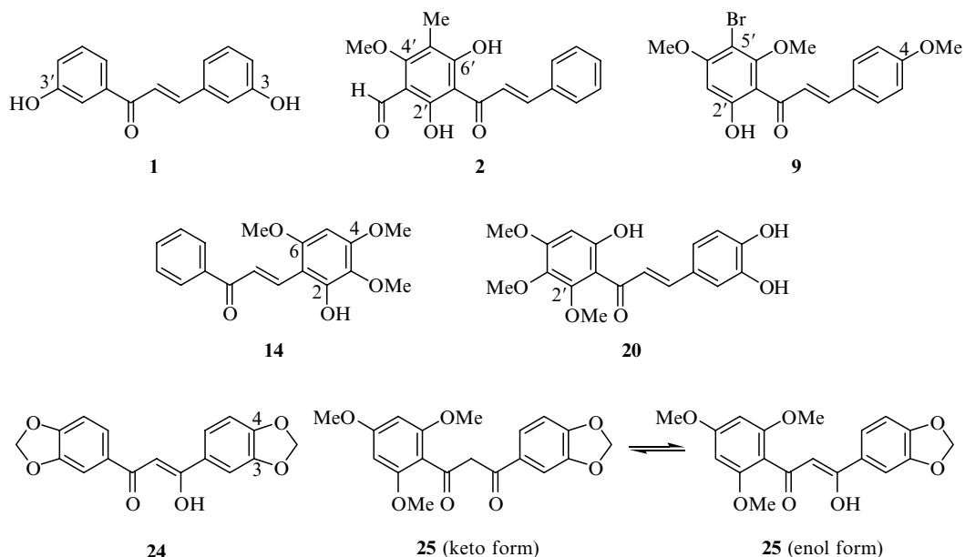
FIGURE 16.6 Chalcones with simple patterns of O -substitution (see Table 16.1).
