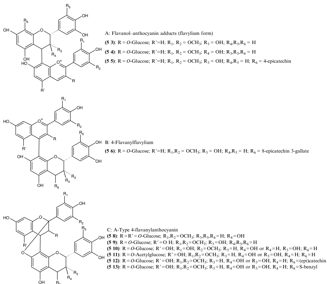
FIGURE 5.7 Structures of anthocyanin–flavanol and flavanol–anthocyanin adducts.
