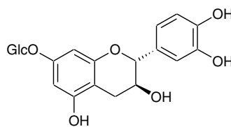
(78)
