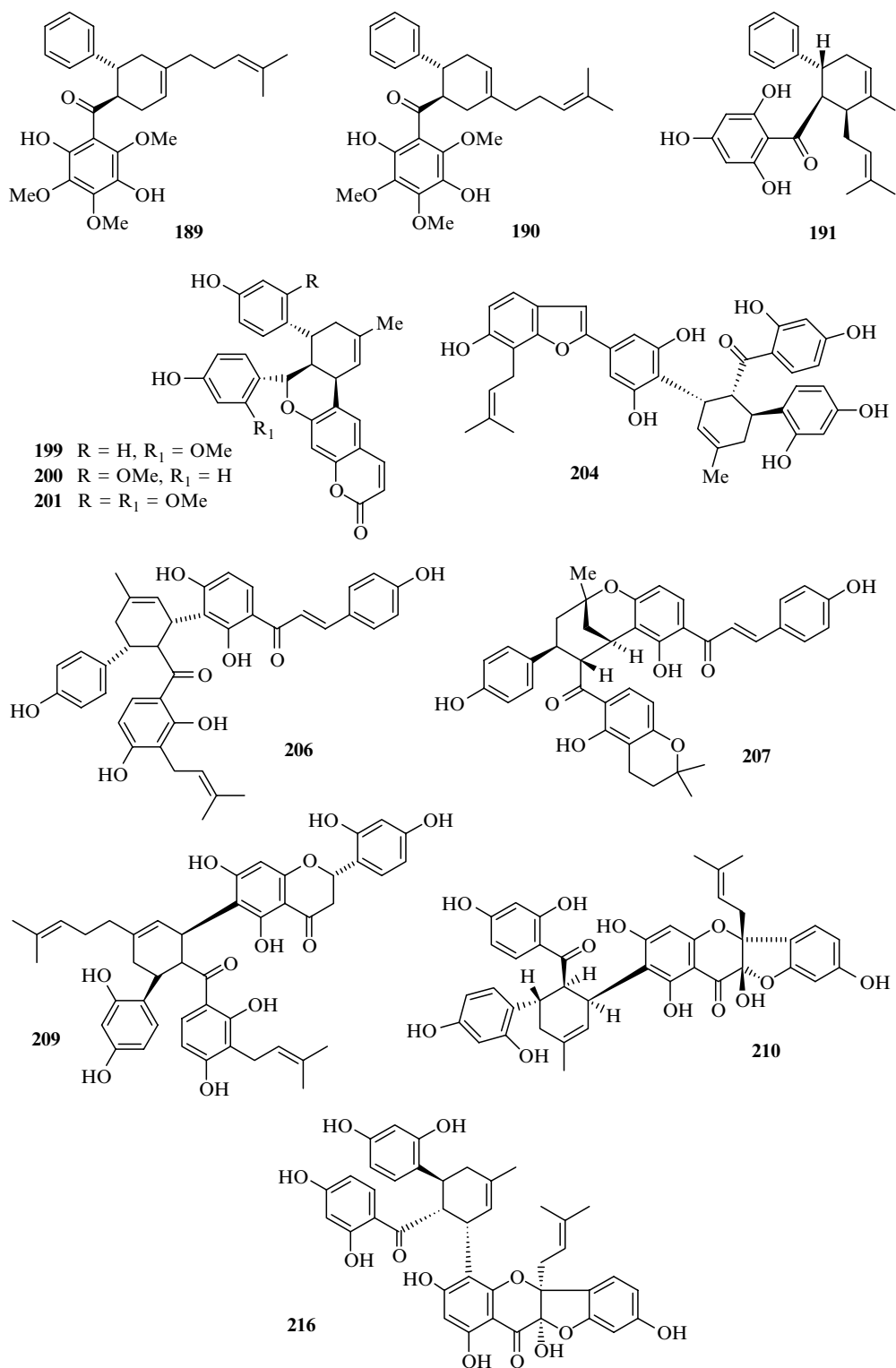
FIGURE 16.11 Diels–Alder adducts of chalcones (see Table 16.5).
