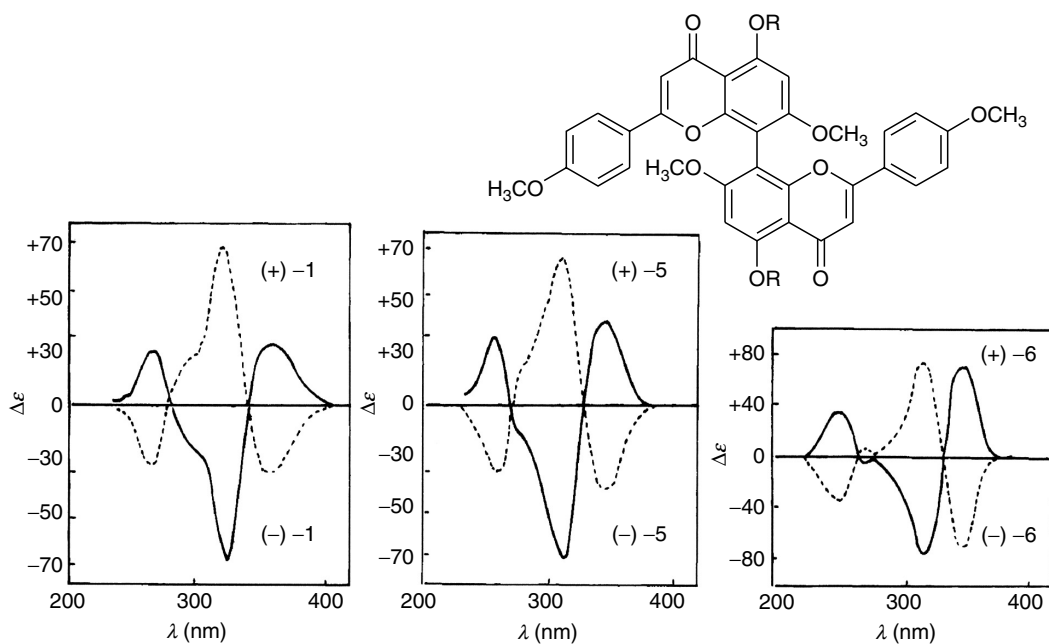
FIGURE 2.23 CD spectra of optically pure 8,8''-biflavones 5,5''-dihydroxy-4,4''',7,7''-tetramethoxy-8,8''-biflavone (1; R = H), its camphorsulphonate derivative (6; R = camphorsulphonate), and its dimethyl derivative, namely 5,5''-dihydroxy-4,4''',7,7''',5,5''-hexamethoxy-8,8''-biflavone (5; R = Me) ( c 8 μg/ml, ethanol). These biflavones are optically active due to the atropisomerism of the biflavone moiety. The dashed lines refer to (+)-1, (+)-5, and (+)-6. The solid lines refer to (-)-1, (-)-5, and (-)-6. Cotton effects observed in the 240 to 360 nm spectral region are similar for the 8,8''-biflavones with the same configuration and independent of the substituents. (Reprinted from Zhang, F.J., Lin, G.Q., and Huang, Q.C., J. Org. Chem. , 60, 6427, 1995. Copyright 1995 American Chemical Society. With permission.)
