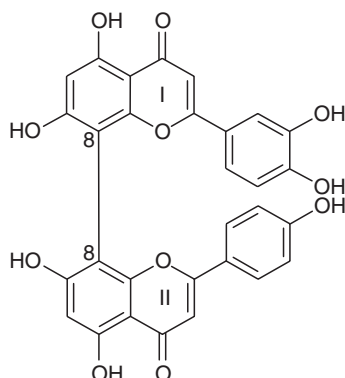
(73) Mogathin (I-3'-hydroxycupressuflavone) — Glossostemon bruguieri (Desf.), Ref. 9
