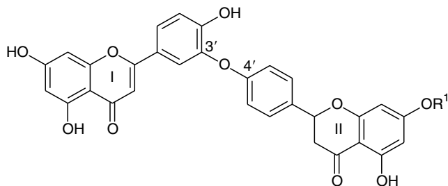
(102) R¹ = H — Luxemburgia nobilis (EICHL), rel. config., Refs. 14, 77
