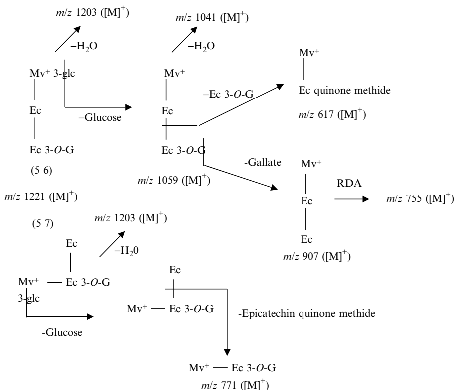
FIGURE 5.8 Mass fragmentation patterns of malvidin 3-glucoside–procyanidin B2 3'-gallate adducts.
