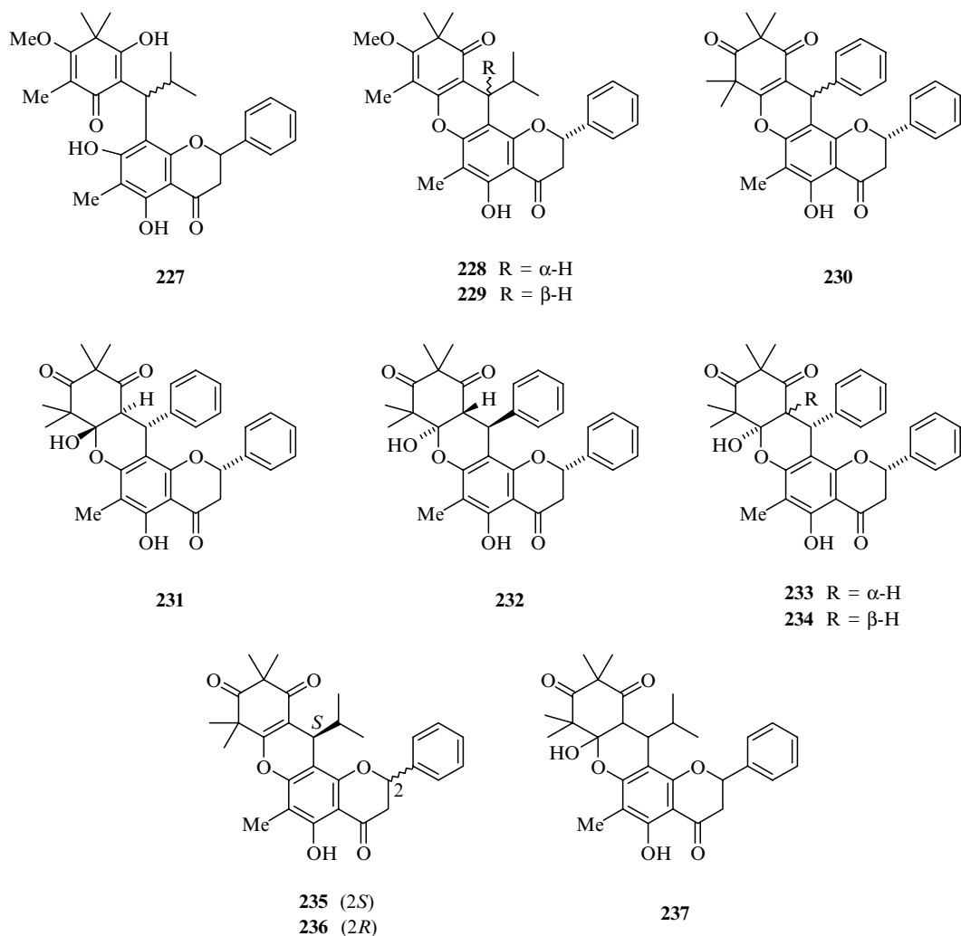
FIGURE 15.9 Complex Myrtaceae flavanones.
