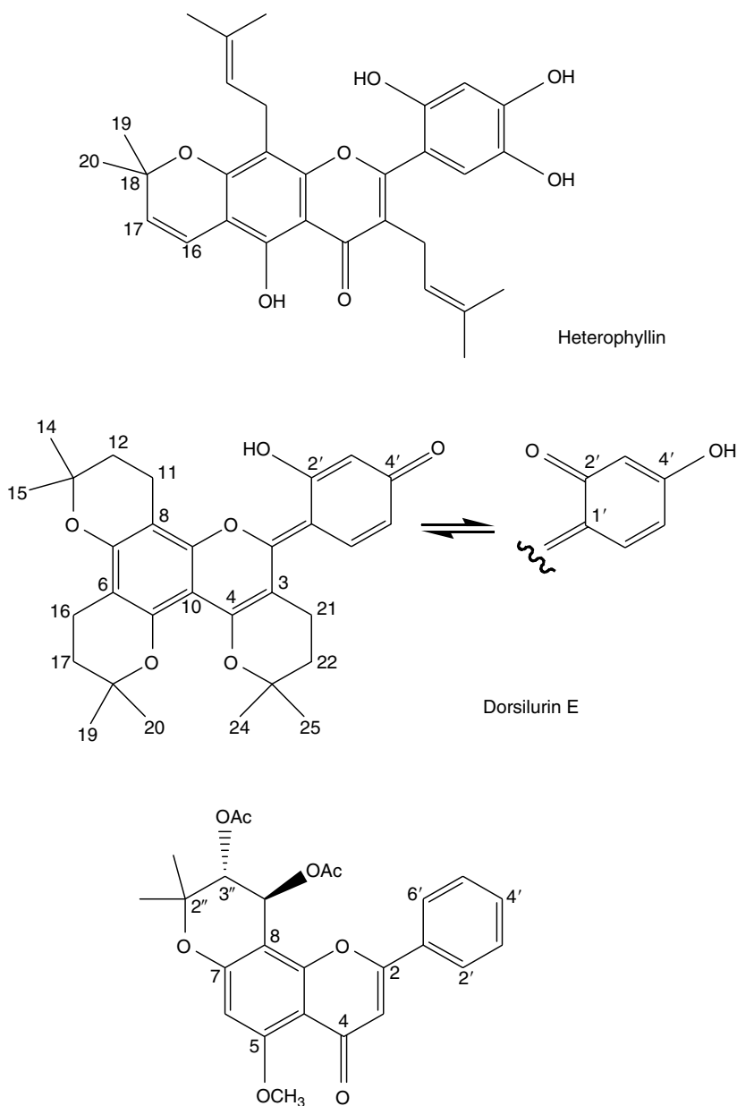
FIGURE 12.2 (Dihydro-) pyranoflavones.
