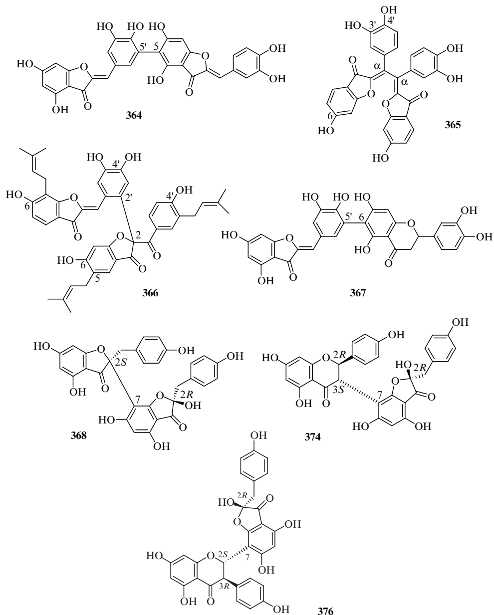
FIGURE 16.21 Aurone and auronol dimers and heterodimers (see Table 16.15).
