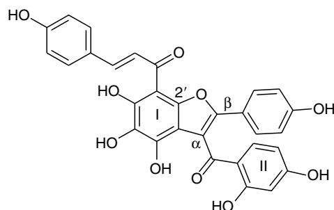
(36) Flavumone A — Oureatea flava , Ref. 64
