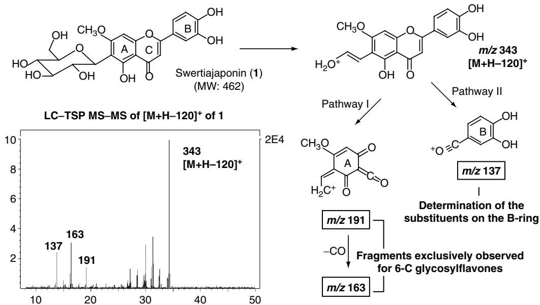
FIGURE 1.9 Online LC-TSP MS-MS of swertiajaponin (1) from the methanol extract of Gentianaella cabreræ . The CID of the [M + H - 120]^+ ion at m/z 343 exhibited characteristic fragments for the substitution of the B-ring and for the glycosylation at C-6. (From Hostettmann, K., Wolfender, J.L., and Rodriguez, S., Planta Med. , 63, 2, 1997. With permission.)
