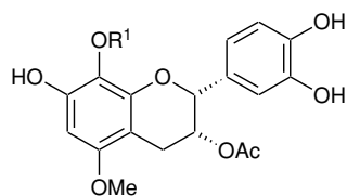
(72) R^1 = \beta\text{-D-glucopyranosyl}
